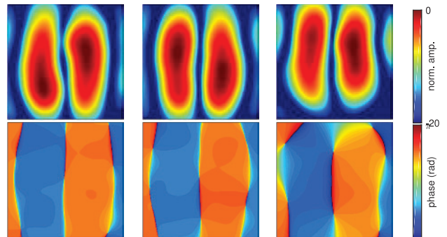
Figure 5: Amplitude (top) and phase (bottom) of the plate mode No 2; Left: 165 Hz (Case 1); Middle: 164 (Case 2); Hz; Right: 173 Hz (Case 3)
