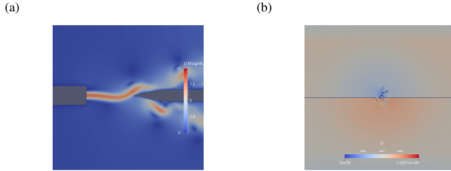
Figure 9. Result of LES at U=5.3\text{m/s} , \Delta x_{min} = 0.05\text{mm} . (a) Velocity distribution. (b) Pressure distribution.
