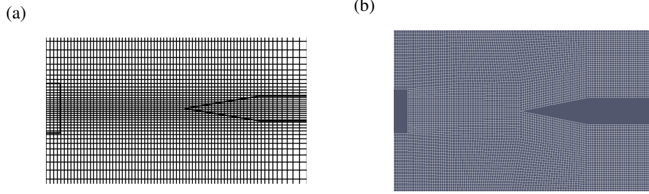
Figure 3. Mesh of DNS and LES : (a) DNS mesh at U=3.3\text{m/s} . The lines are drawn every 10 grid intervals. (b) LES mesh with x_{min} = 0.1\text{mm} .
