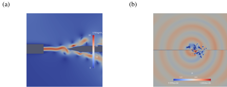
Figure 10. Result of LES at U=16.7\text{m/s} , \Delta x_{min} = 0.05\text{mm} . (a) Velocity distribution. (b) Pressure distribution.
