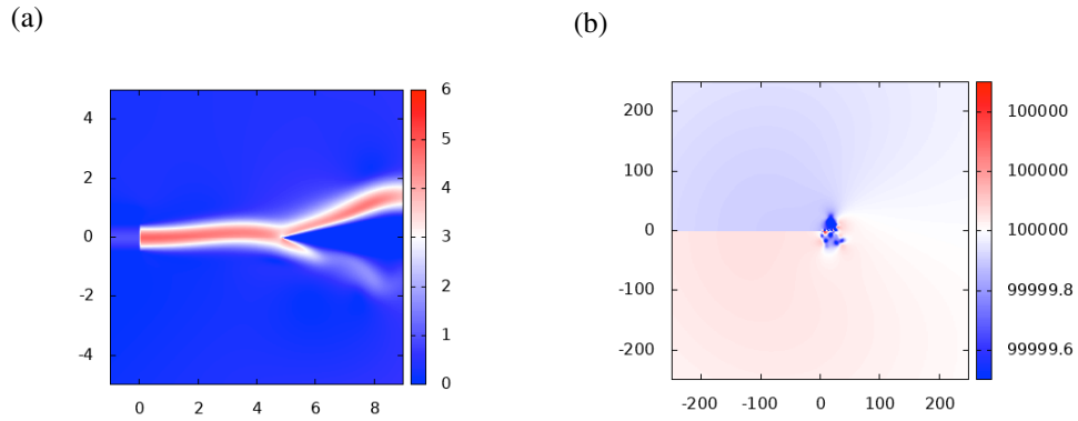
Figure 4. Result of DNS at U=4.7\text{m/s} . The unit of the horizontal and vertical axes is mm. (a) Velocity distribution. (b) Pressure distribution.
