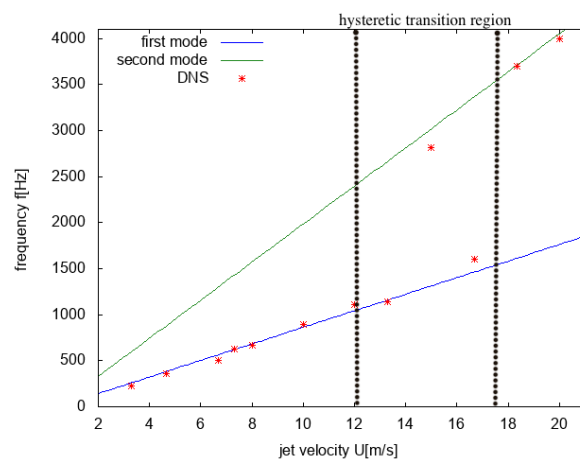
Figure 6. Results of DNS : frequency vs jet velocity. Blue and green lines are first and second modes obtained by Brown's equation (1), respectively. The vertical dotted lines indicate the lower and upper limits of the hysteresis transition region.
