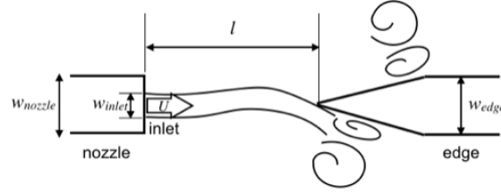
Figure 1. Edge tone : In the 2D model, the parameters are taken as l = 5\text{mm} , w_{edge} = 1.2\text{mm} , w_{nozzle} = 1.2 , w_{inlet} = 1\text{mm} .
