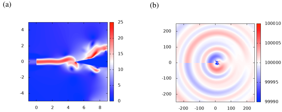
Figure 5. Result of DNS at U=18.3\text{m/s} . (a) Velocity distribution. (b) Pressure distribution.
