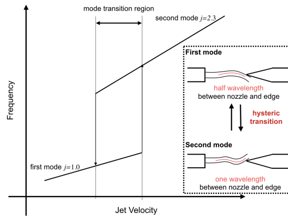
Figure 2. Hysteretic mode transition of edge tone.
