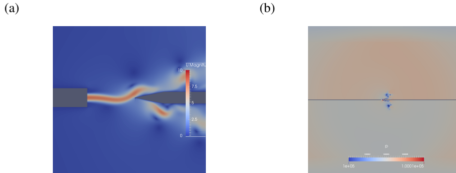
Figure 7. Result of LES at U=5.3\text{m/s} , \Delta x_{min} = 0.1\text{mm} . (a) Velocity distribution. (b) Pressure distribution.
