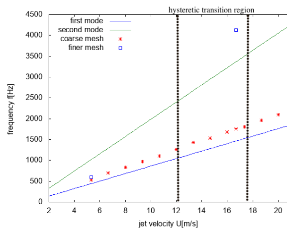
Figure 11. The frequencies obtained with LES for the coarse and finer grained meshes together with the first and second modes of Brown's equation.
