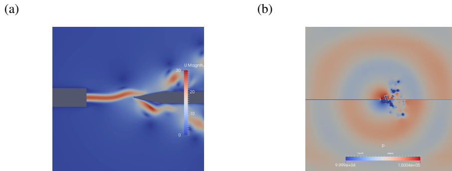
Figure 8. Results of LES at U=16.7\text{m/s} and \Delta x_{min} = 0.1\text{mm} . (a) Velocity distribution. (b) Pressure distribution.
