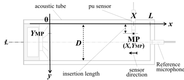
Figure 3. Acoustic tube for PU-sensor calibration. End walls are openable for the purpose of ventilation.[7]
