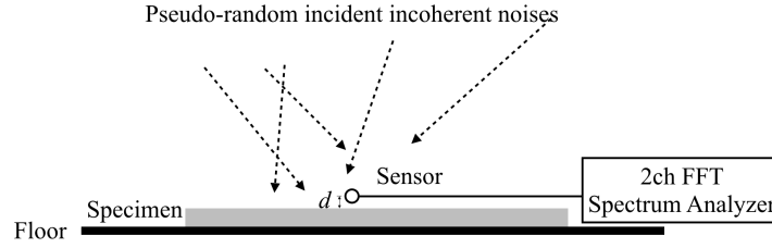
Figure 1. Measurement setup of the EA method. At the sensor position, EA pu method sets PU-sensor; and EA pp method sets two-microphone. Sensor is located d m above the specimen surface.
