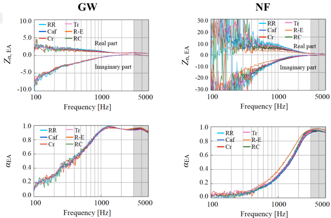
Figure 6. Sound absorption characteristics of GW (left column) and NF (right column) measured by EApu method at six sound fields (RR, Caf, Cr, Tr, R-E, RC). Mean values over nine-times repetition in each sound field are plotted. (upper row): surface normal impedance; and (lower row): absorption coefficient.
