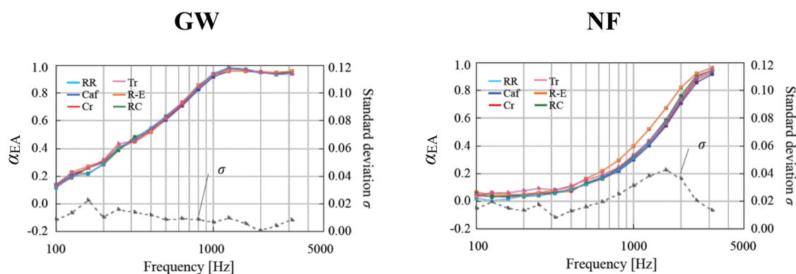
Figure 7. Comparisons of 1/3 octave band mean values of \alpha_{EA} of GW and NF between six sound fields (RR, Caf, Cr, Tr, R-E, RC). Standard deviation \sigma values are plotted together with right axis.
