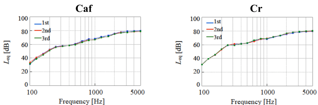
Figure 5. Frequency characteristics of L_{eq,20s} measured by sound level meter during the three-day (1st, 2nd and 3rd) EA pu method measurements. Microphone of the sound level meter was placed at the specimen's center point close to PU-sensor. The measurements were conducted in the sound fields Caf (Left) and Cr (Right).
