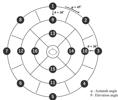
Figure 6. Arrangement of sound sources in the second experiment.
