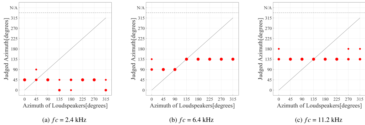
Figure 4. Localization test results of narrowband signal (Right ear hearing)
