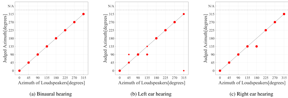
Figure 3. Localization test results of broadband signal
