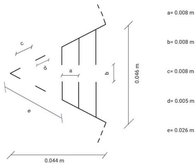
Figure 3 – Dimensions of the metamaterial unit formed in the folded state for Design 1.
