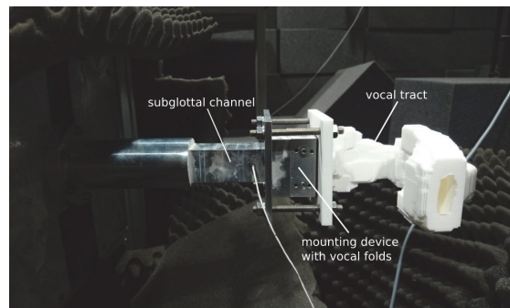
Figure 2. Experimental setup with subglottal channel, artificial vocal folds, and MRI-based vocal tract
