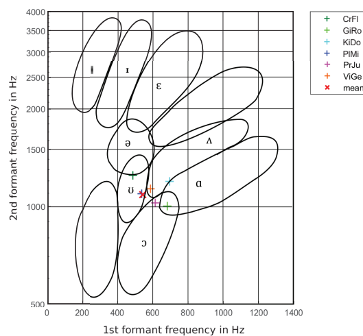
Figure 5. The formant chart, according to Peterson and Barney [14] shows the formant frequencies of the mean vocal tract compared to the physiological formants of the tenors.
