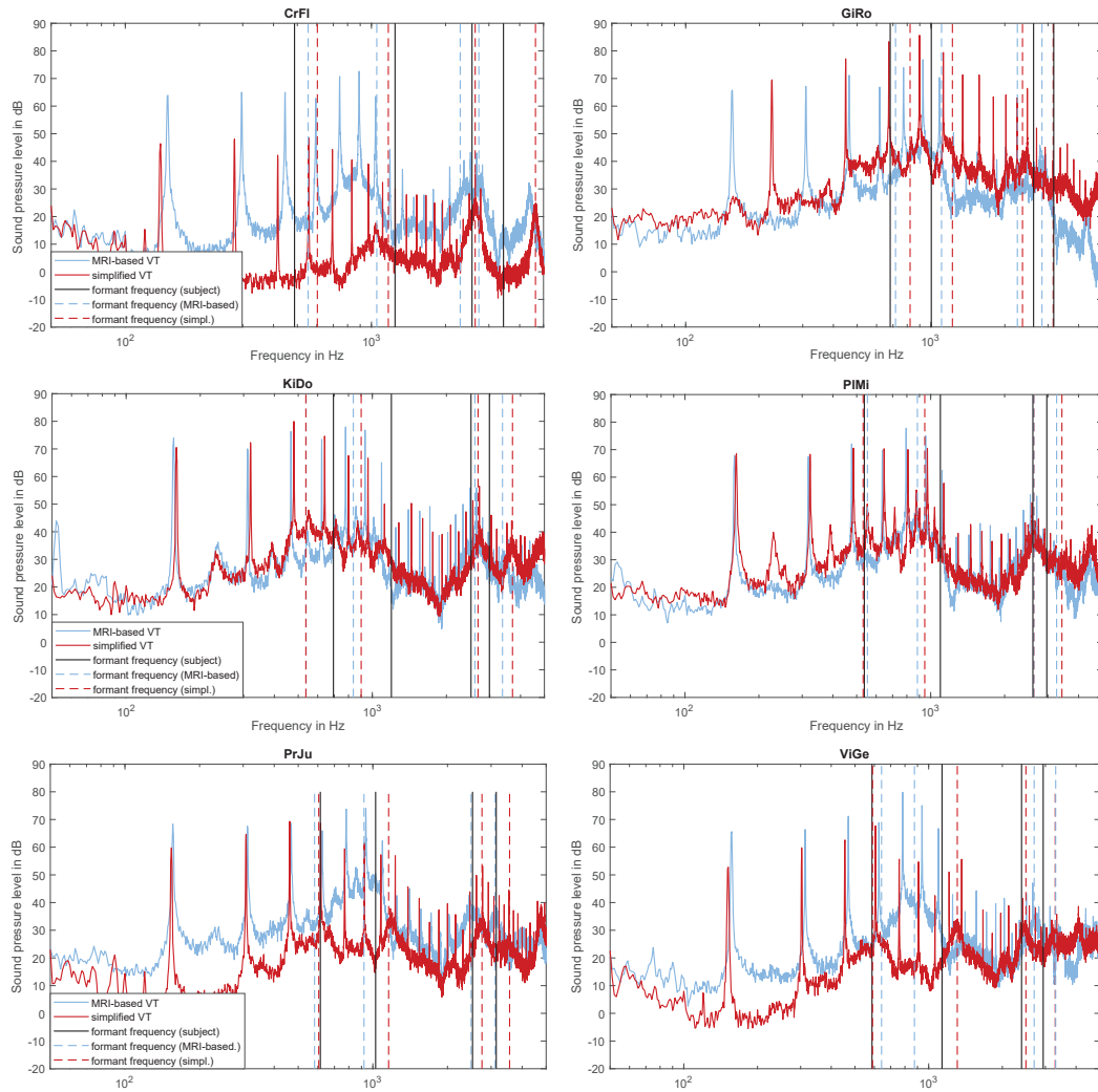
Figure 3. Sound pressure level of the MRI-based (blue) and simplified (red) models for all subjects. The formant frequencies, as detected by inverse filtering are marked with vertical lines
