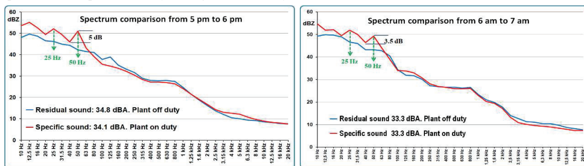
Figure 7 – Spectrum comparison on different hours. Plant on duty vs. off duty (re dB 20 µPa)
