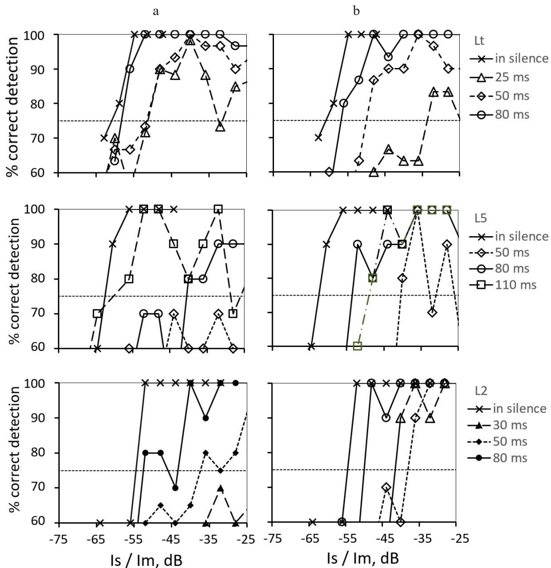
Figure 2. – Dependent of correct detection of test pulse on ratio of the test pulse level to pulse train level. (a) test pulse before the pulse train (b) test pulse after the pulse train. Data for “typical” listeners with normal hearing (Lt), “untypical” listener with normal hearing (L5) and listener with aging-related hearing loss (L2).
