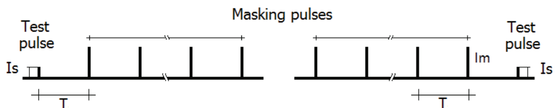
Figure 1. – Temporal diagrams with the test pulse before the pulse train (left) and after the pulse train (right).
