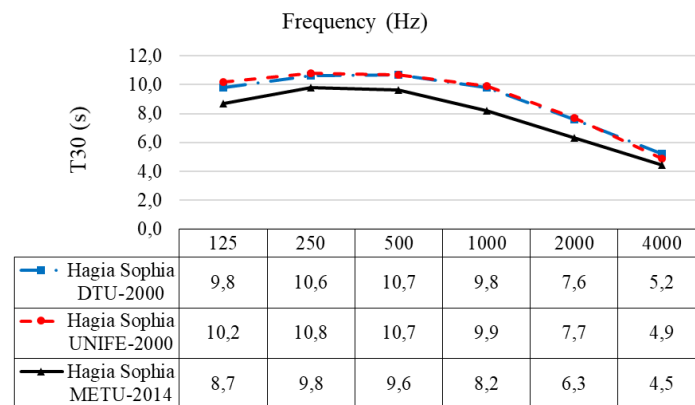
Figure 5. Comparison of T30 field test results of Hagia Sophia by DTU-2000, UNIFE-2000 and METU-2014 in field tests, in 1/1 octave bands from 125 Hz to 4000 Hz.
