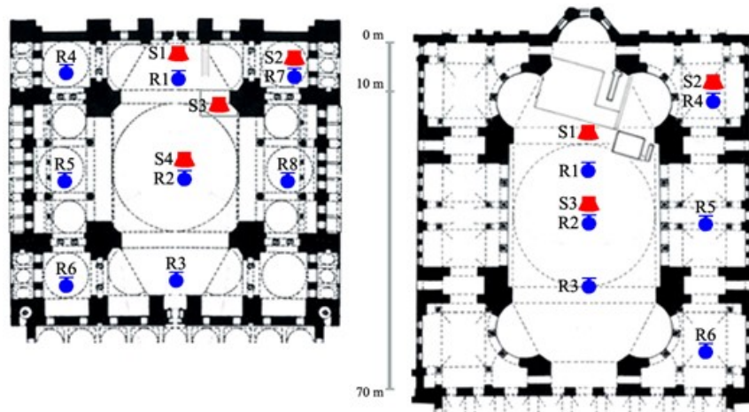
Figure 3 - Plan views with sound Source (in red) and Receiver (in blue) locations of METU- 2013 field tests in Süleymaniye Mosque (on the left) and METU-2014 field tests in Hagia Sophia (on the right)
