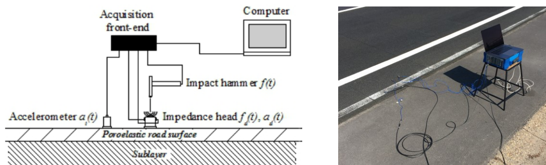
Figure 6 – (left) Procedure for the determination of the mechanical impedance (14) – (right) Actual setup
