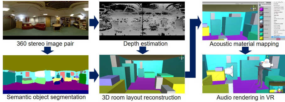
Figure 1. Overview of the audio rendering from visual captures.
