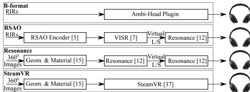
Figure 2. Overview of the four methods used to generate the stimuli.
