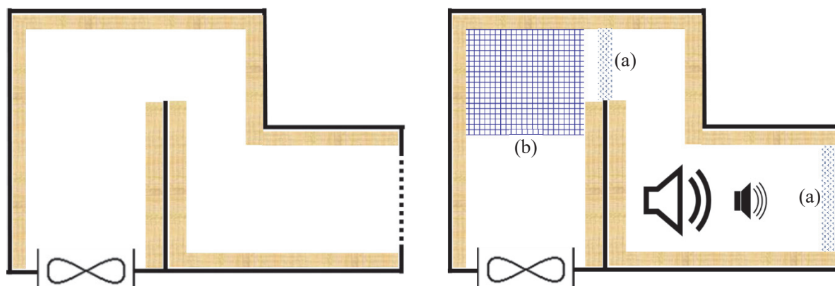
Figure 6 – Construction of the enclosure as recommended by manufacturer (left) and supplemented by additional absorbing material and a loudspeakers of an ADC system
