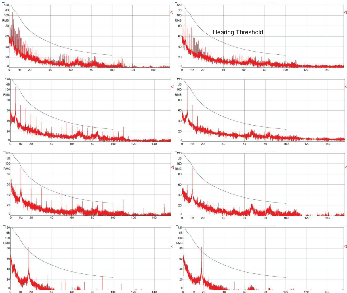
Figure 8 – Spectrum of the sound pressure of the scenarios 1 to 4 (top down) without (left) and with (right) ADC
