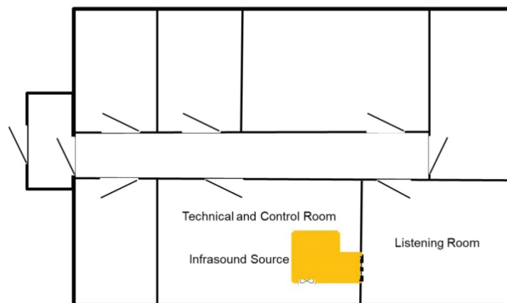
Figure 2 – Layout of the test house
