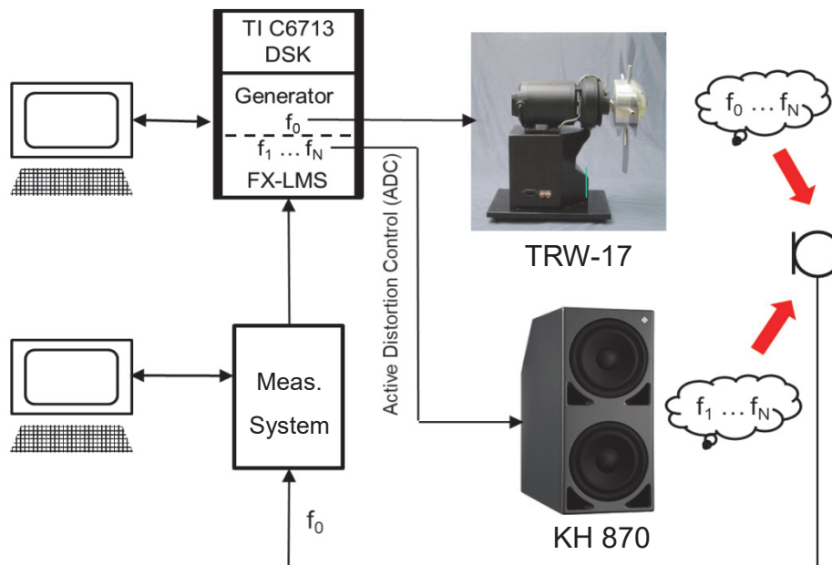
Figure 7 – Conceptual structure and operation of the ADC system
