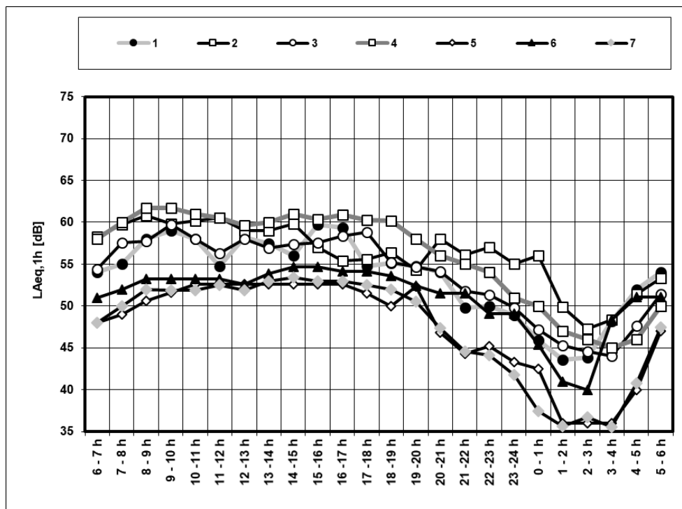
Fig. 2. The course of L_{Aeq/1h} measurements on noisy facades more then approximately 100 meters from noisy traffic communications and inner city corridors (numbers from 1 to 7 according the table 2)
