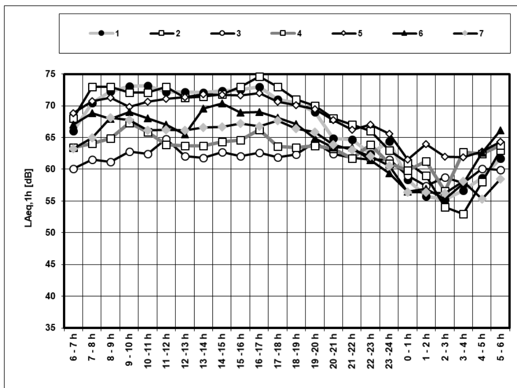
Fig. 1. The course of L_{Aeq,1h} measurements on noisy facades up to 50 meters from noisy traffic communications (numbers from 1 to 7 according the table 1)
