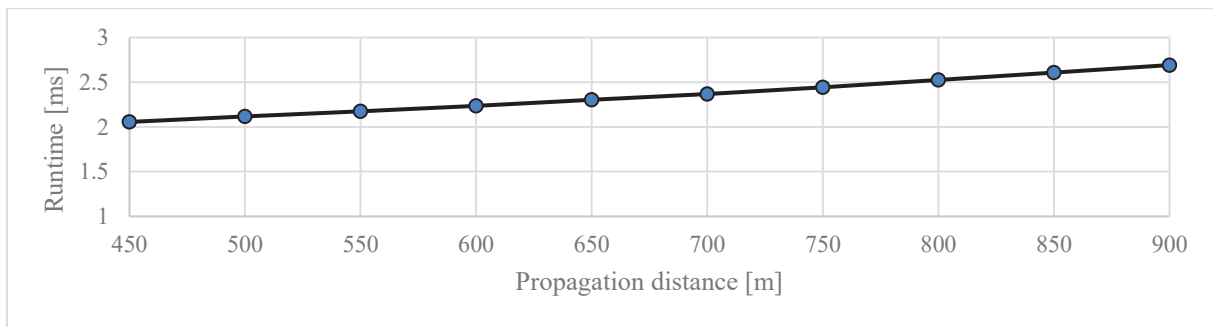
Figure 6: Runtime for increasing culling distance at constant number of buildings.
