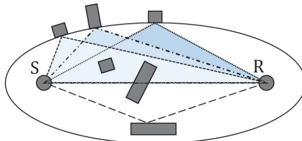
Figure 2: Cross-section of the propagation constraint of maximum detour reduced to a 2D ellipse problem.
