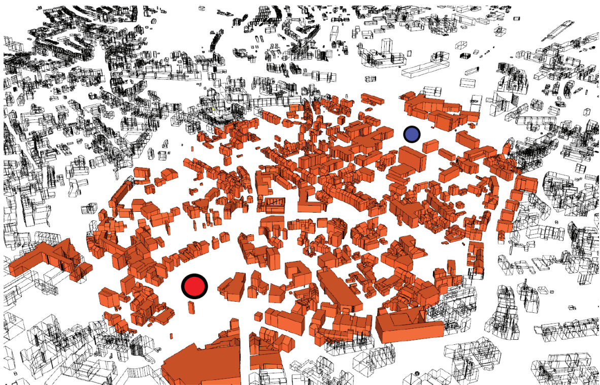
Figure 4: Visualization of the acoustics-driven geometry filtering algorithm applied to a real urban data set. To emphasize the resulting ellipsoidal shape, an exaggeratedly loud sound source has been used.
