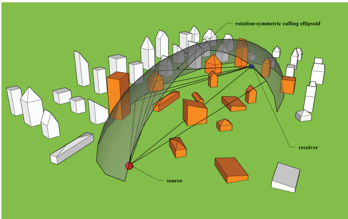
Figure 1: Culling ellipsoid for a source-receiver-pair in an urban environment.
