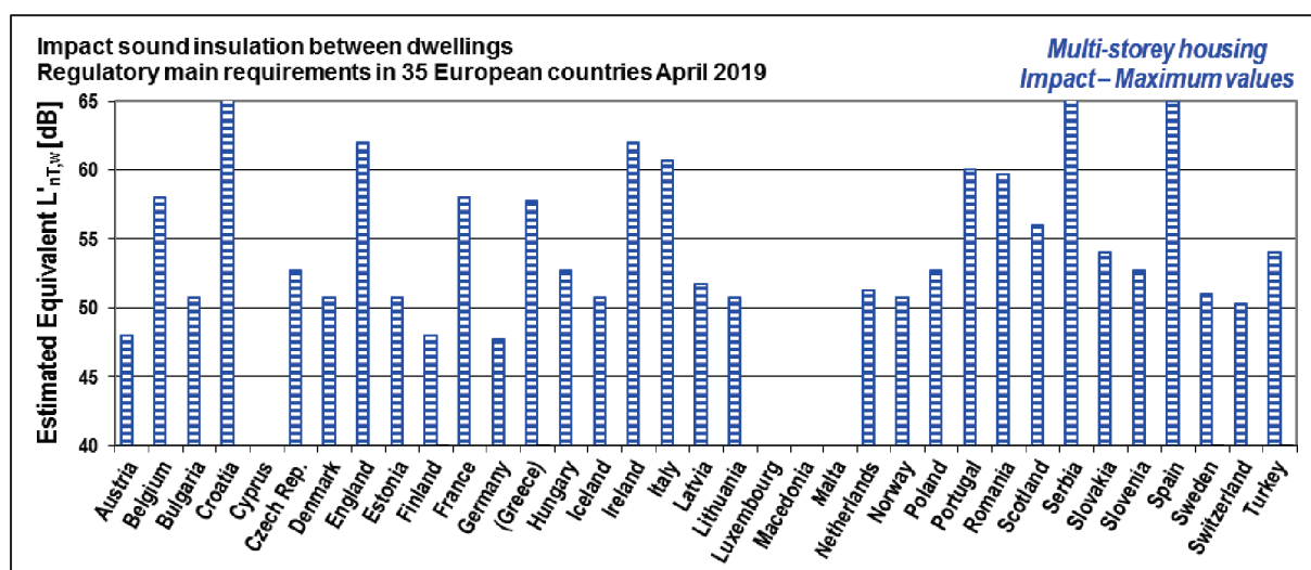
Figure 2 – Overview of impact sound insulation requirements between dwellings. Status April 2019. Graphical presentation of estimated equivalent values of L'_{nT,w} . Note: The equivalent values are estimates only, as exact conversion is not possible.
