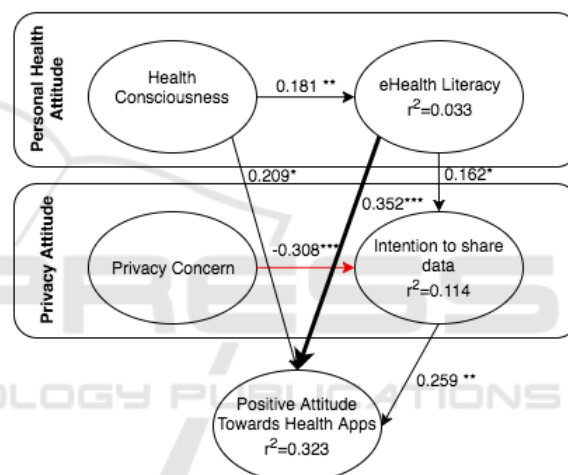
Figure 3: Results of the PLS-SEM Algorithm. Only significant paths (after bootstrapping) are shown. Red arrows indicate negative path coefficients.
