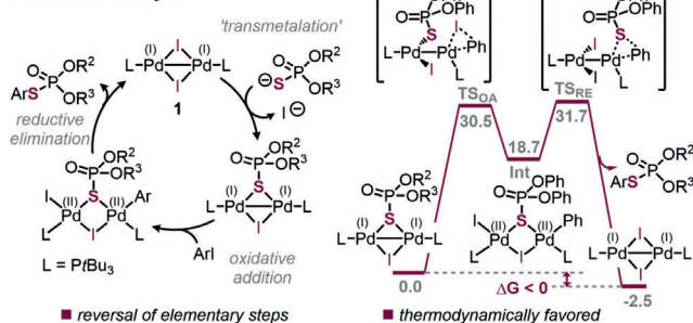
Figure 1. Free energy profile of Pd I -catalyzed coupling of PhI with [SP(O)(OPh) 2 ] − . Gibbs free energies (in kcal mol −1 ) shown, calculated at the SMD (toluene) M06L/def2TZVP//B3LYP-D3/6-31G(d, p) (SDD for Pd, I) level of theory.
