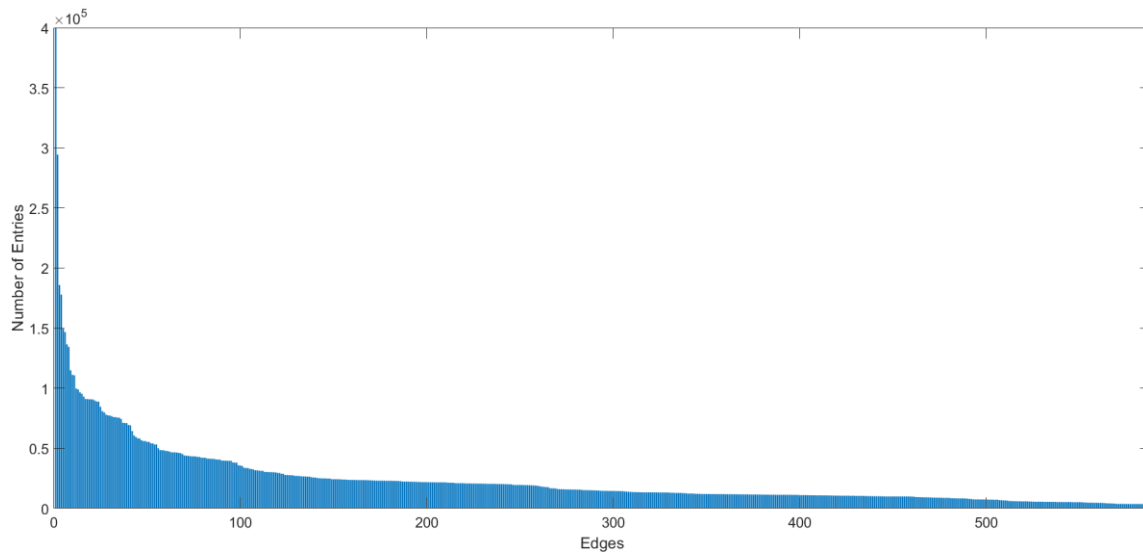
Figure 4: Number of entries for the observed edges in decreasing order
