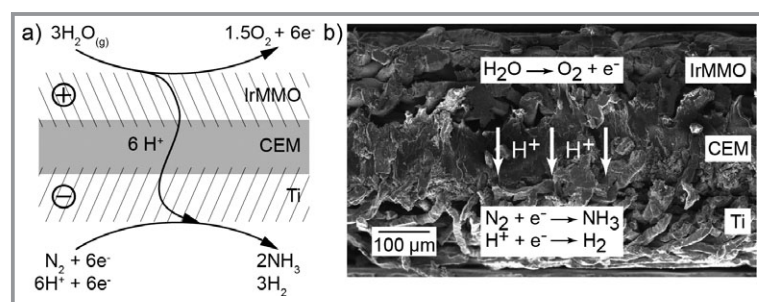
Figure 1. a) Visualization of reactions at the MEA: at the anode, \text{H}_2\text{O} is oxidized to form \text{O}_2 and electrons, \text{H}^+ migrates through the CEM to the cathode where it combines to \text{H}_2 or \text{N}_2 is reduced to \text{NH}_3 . b) SEM image of the MEA consisting of an IrMMO anode, the CEM and a Ti cathode.
