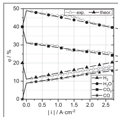
Figure 2. Comparison of output gas composition for the initial mixture 40 % \text{H}_2\text{O} + 40 % \text{CO}_2 + 20 % \text{H}_2 at 900^\circ\text{C} and a flow rate of 6 \text{ L h}^{-1} between experimental results (transparent symbols) and theoretical calculations (filled symbols) up to an operation of 2.7 \text{ A cm}^{-2} .
