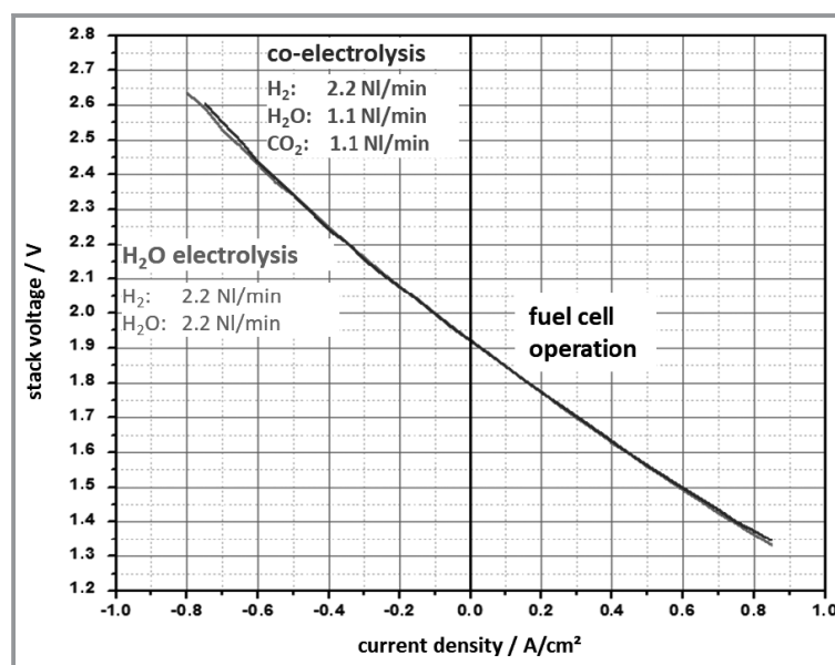
Figure 1. Current-voltage characteristics for a 2-cell short stack operated at 800 °C in both fuel cell and electrolysis mode with 50 % H_2O + 50 % H_2 (steam electrolysis) and 25 % H_2O + 25 % CO_2 + 50 % H_2 (co-electrolysis) as feed gas.
