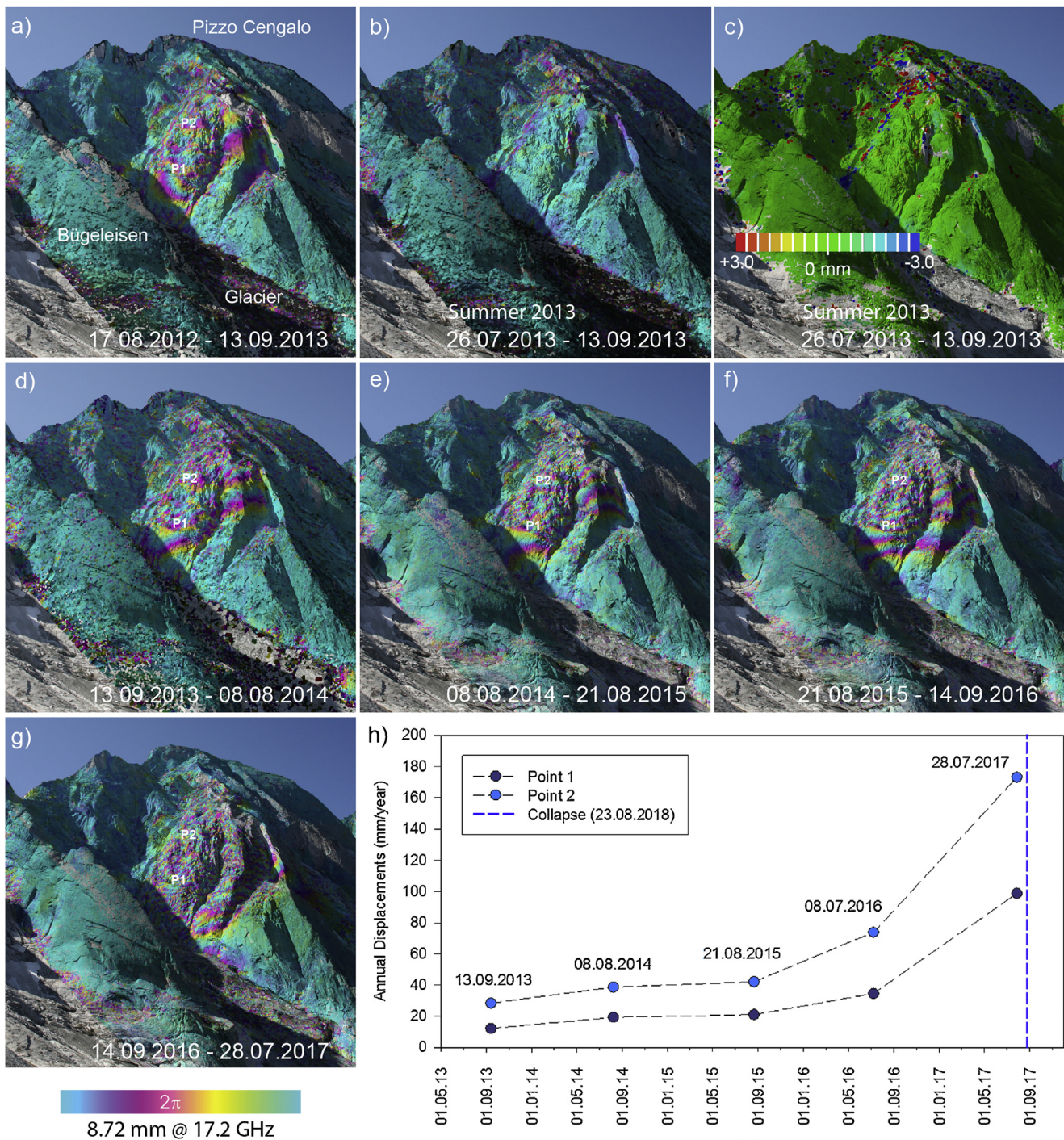
Fig. 4. Results of rock slope displacement monitoring acquired with a portable radar interferometer. Displacements in panels a, b, d – g are shown as interferograms. Each color cycle (e.g., fringe) represents an 8.72 mm displacement and is defined by the wavelength of the radar's central frequency (e.g., 17.2 GHz). c, a phase-unwrapped displacement map, scaled to \pm 3.0 mm. The interferograms and displacement map were projected into a three-dimensional photogrammetric model for visualization. At points P1 and P2 displacement data were extracted and plotted in panel h. h) yearly displacement rates at two selected points extracted from interferograms between 2012–2017 (P1 and P2). The date of catastrophic failure is shown by the dashed line.
