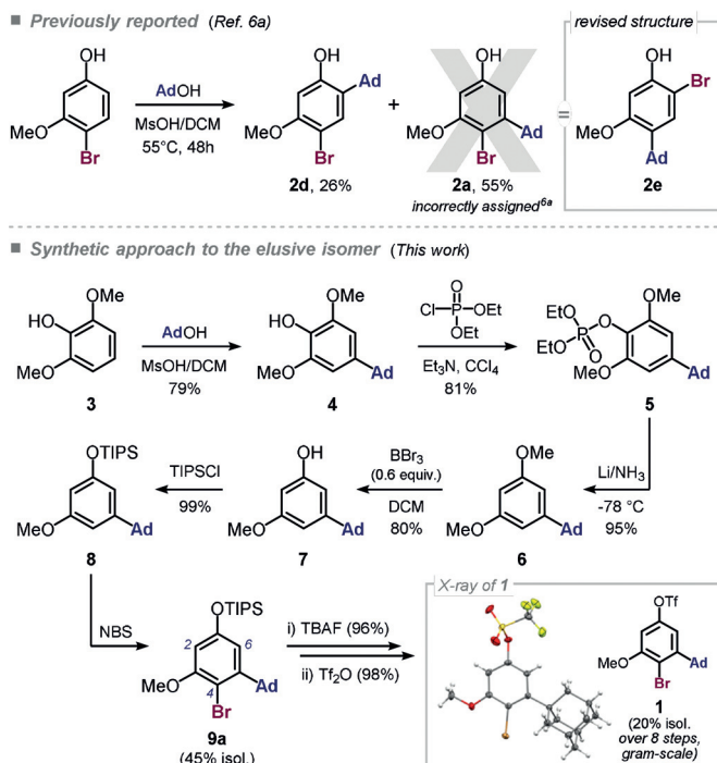
Scheme 1. Structural revision of previously claimed ortho -bromo-adamantylarene ( 2a ) and synthesis of 4-bromo-5-methoxy-3-adamantyl-phenyl triflate ( 1 ) from 1,3-dimethoxyphenol 3 . See the Supporting Information for detailed reaction conditions.
