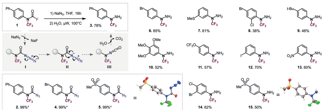
Figure 2. Proposed mechanism for the formation of hydrazines; *yield of carbamoyl azides after filtration; prepared N -CF 3 hydrazines (3, 6–15) and X-ray structures. [17]
