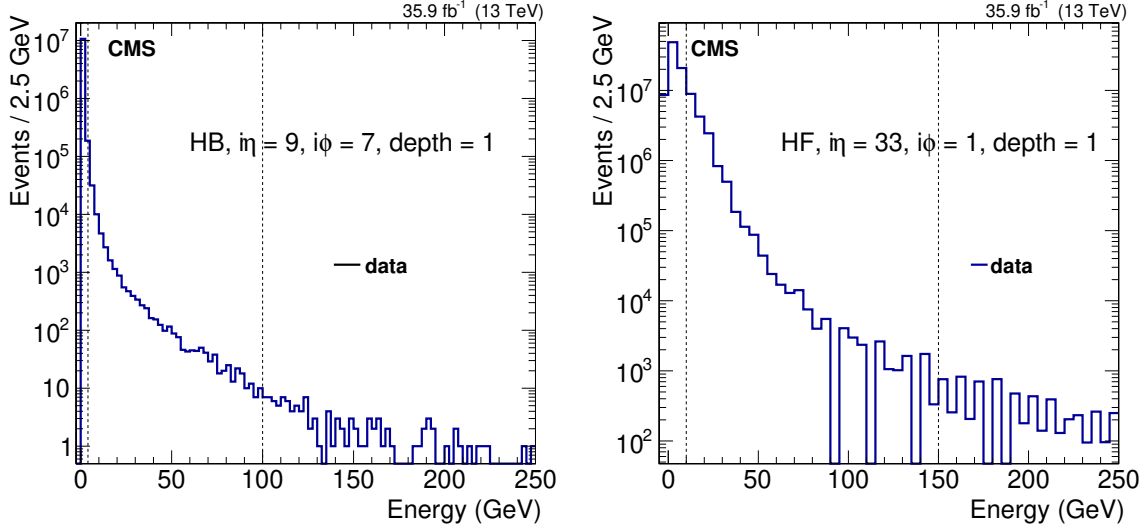
Figure 2. Energy spectra used as an input to the iterative method of equalizing the \phi response of one typical i\eta ring for an HB (left) and HF (right) calorimeter channel. Thresholds on the collected energies used for the energy estimation are shown with dashed lines. The legends show the HCAL channel index in i\eta , i\phi , and depth segmentation units.
