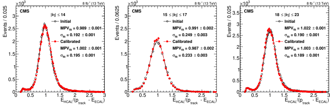
Figure 9. Response distributions for pions from 2016 data in three different \eta regions, |\eta| \leq 1.22 (left), 1.22 < |\eta| \leq 1.48 (middle), and 1.48 < |\eta| \leq 2.04 (right), with loose charged-particle isolation criterion: initial (black circles) and after convergence (red squares). Only statistical uncertainties are shown on the data points.
