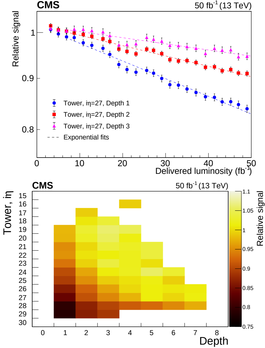
Figure 13. Upper: relative signal F for \eta = 27 in depths 1, 2, and 3 versus delivered luminosity using the in situ “inclusive” method; the dashed lines show the results of fits with an exponential function, after excluding the first 7 \text{ fb}^{-1} of data, as was done in the laser data analysis (section 4.2). For the tile in depth 1 (i.e., layer 0), the estimated dose at the end of data taking was d = 1.5 \text{ kGy} and the average dose rate was R = 0.89 \text{ Gy/h} . Lower: relative signal F for towers with \eta = 16 –29 at different depths measured after 50 \text{ fb}^{-1} of delivered luminosity; only results with a relative uncertainty of 3% or lower on measured values of F are shown. Tiles in depth 1 are made of BC-408 and tiles in other depths are SCSN-81.
