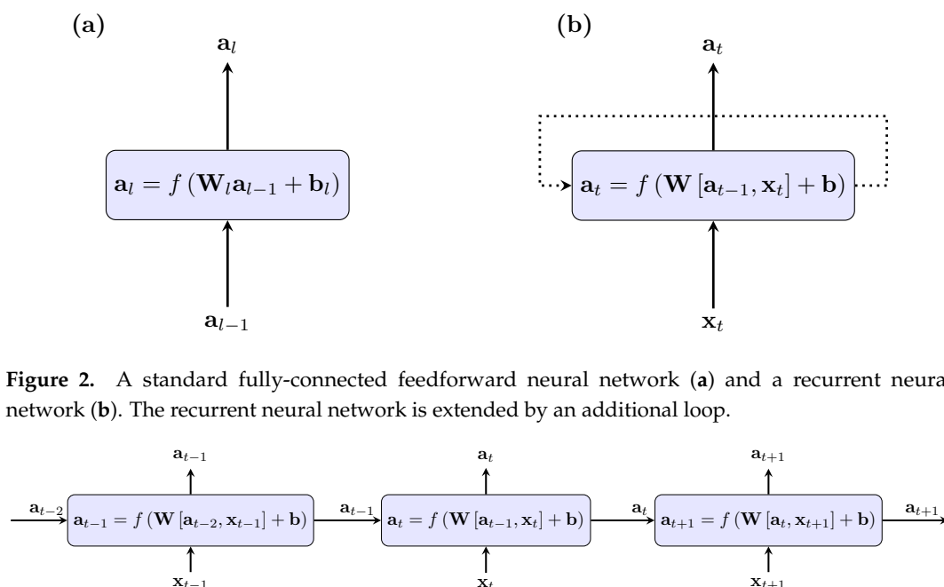
Figure 3. Unfolded view on a recurrent neural network. The neural network is extended by an additional loop which allows the use of previous information for the subsequent prediction.
