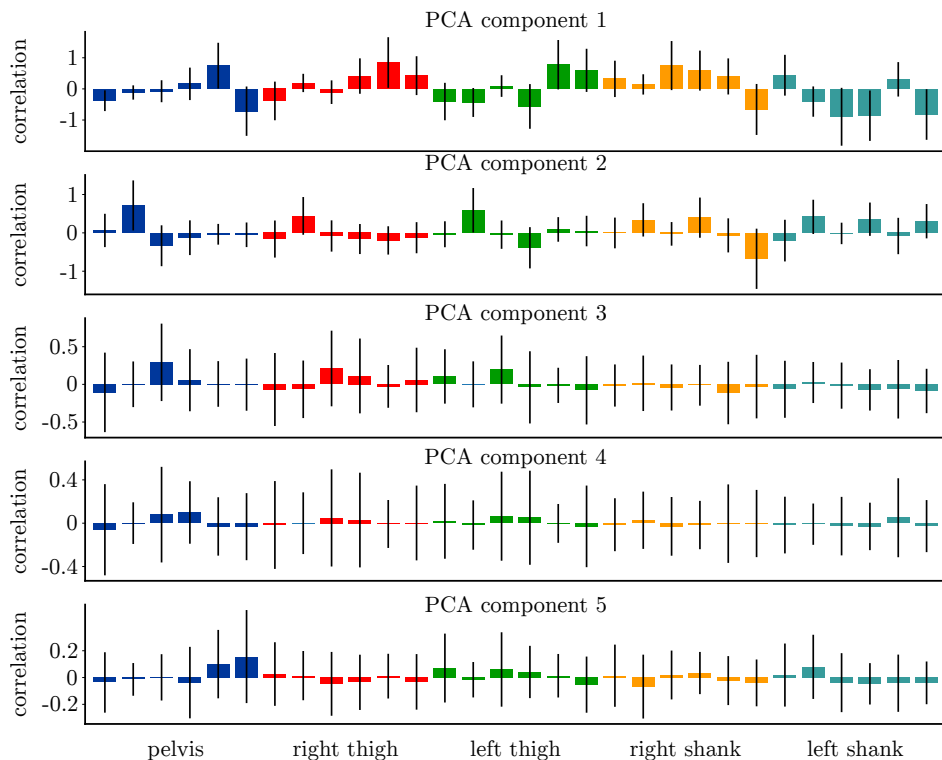
Figure 5. Correlation of each sensor's reading ( acc_x , acc_y , acc_z , \omega_x , \omega_y , \omega_z ) with the first five PCA components. The correlation strength of the acceleration is, in general, less than that the correlation of the angular rate with the single components. The pelvis and shank sensors show stronger correlations with the PCA components than the thigh sensors.
