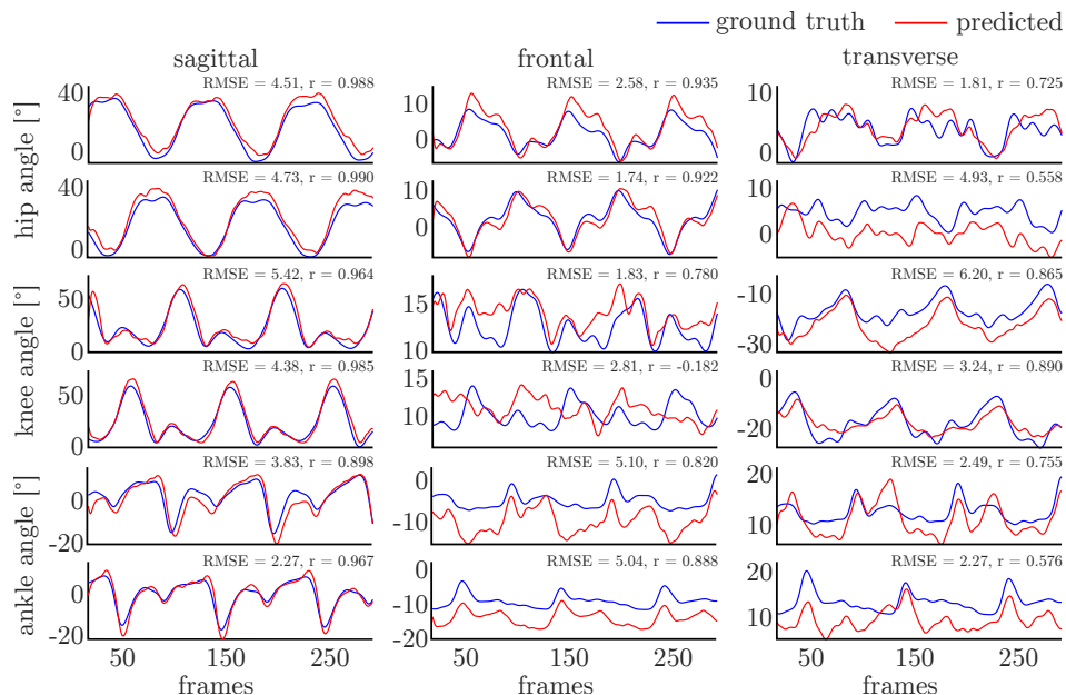
Figure 6. A single example of the joint angle prediction using PCA-net. The joint angles predicted for the right are displayed on top of those predicted for the left. The sample depicts the one with the median RMSE value.
