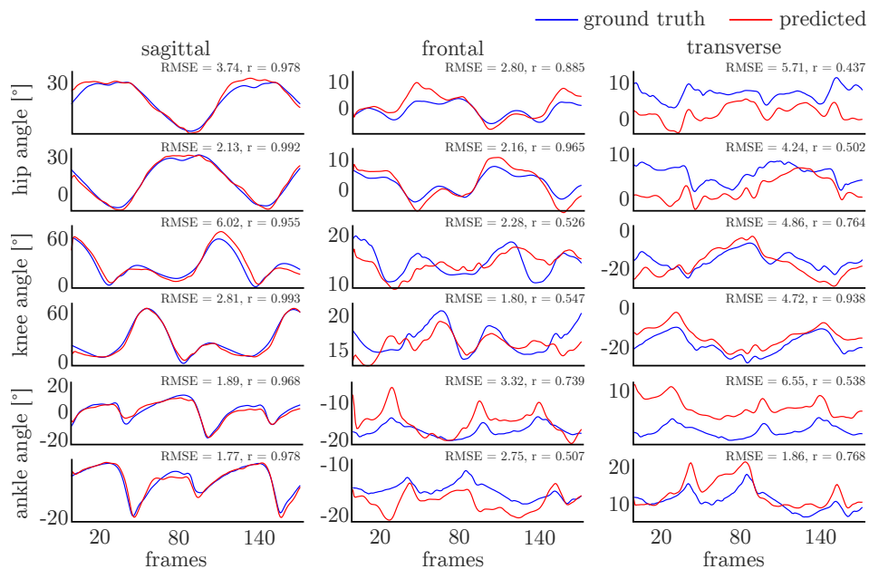
Figure 7. A single example of the joint angle prediction using PS-net. The joint angles predicted for the right are displayed on top of those predicted for the left. The sample depicts the one with the median RMSE value.
