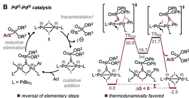
Figure 1. Free energy profile of Pd I -catalyzed coupling of PhI with [SP(O)(OPh) 2 ] − . Gibbs free energies (in kcal mol −1 ) shown, calculated at the SMD (toluene) M06L/def2TZVP//B3LYP-D3/6-31G(d, p) (SDD for Pd, I) level of theory.
