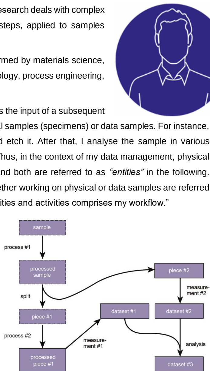
Figure 3.4.1 Provenance graph in the sample-based workflow
