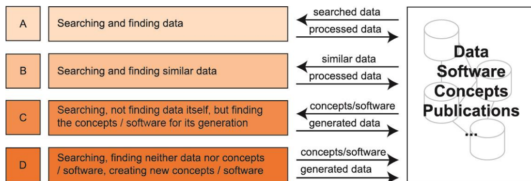
Figure 3.6.1 ELLEN's gradually extended detour to retrieve required data
