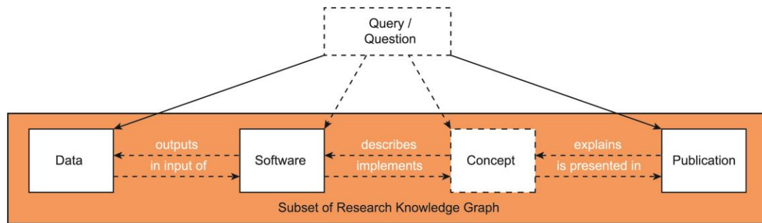
Figure 3.6.2 Subset of Research Knowledge Graph elements relevant for the querying of data generation methodologies (the focus of this task area is indicated by dotted lines)
