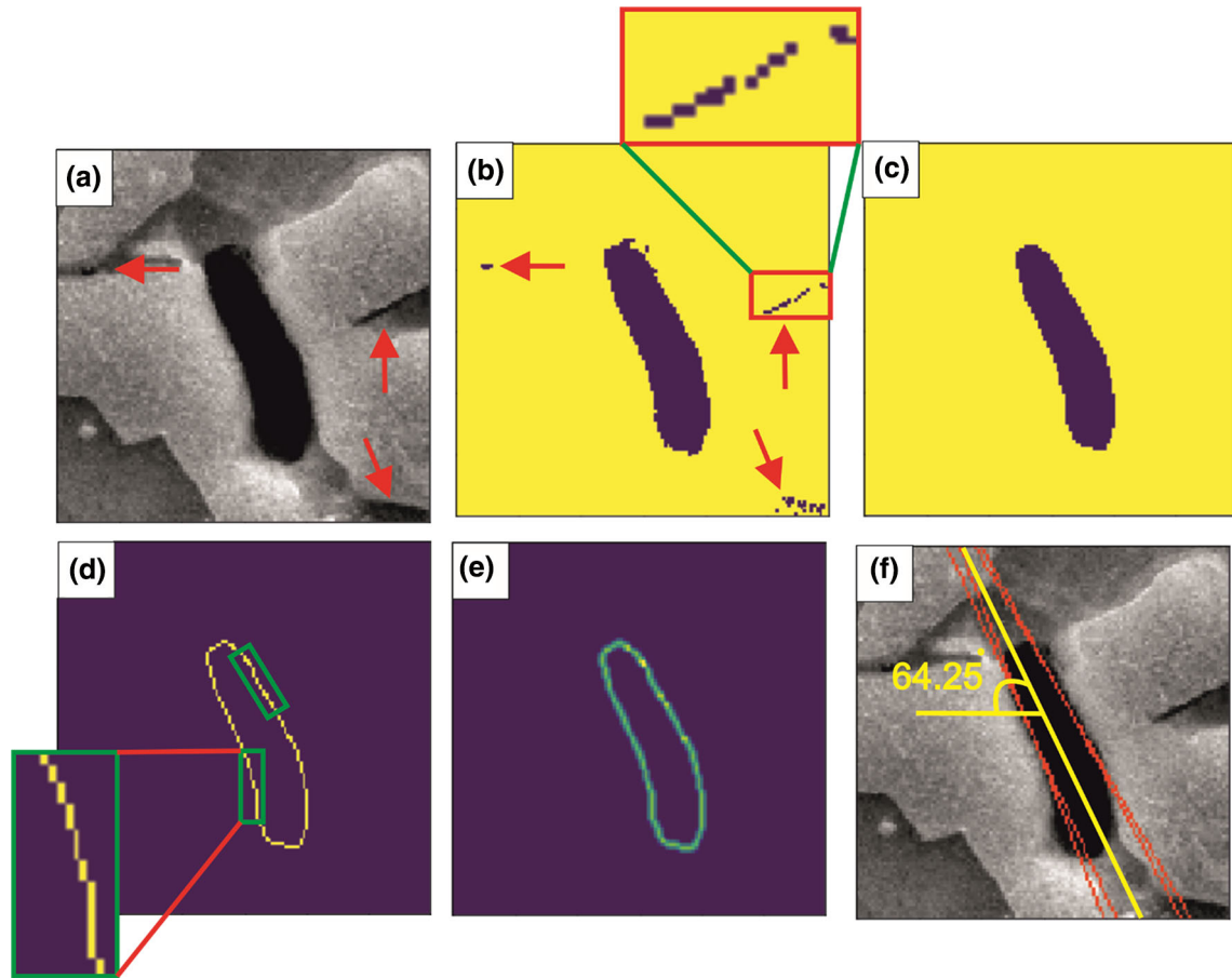
Fig. 3. Martensite crack angle calculation flow: (a) detection of crack, (b) example of noise due to shadowing after thresholding, (c) filtered crack by application of DBSCAN, (d) detection of crack circumference by Canny edge detection, (e) Gaussian blurred edge, and (f) example of lines detected on crack edge overlaid on micrograph.
