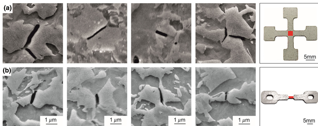
Fig. 1. Comparison between sample geometry and martensite crack orientation appearing in the sample after (a) biaxial and (b) uniaxial tensile testing.
