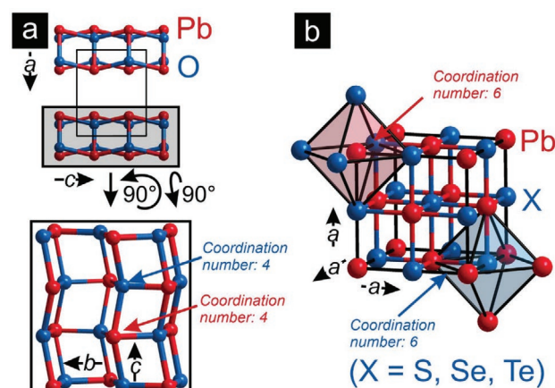
Figure 1. Representations of the crystal structures of a) the massicot-type \beta - PbO and b) the rocksalt-type PbX ( X = S, Se, \text{ or } Te ): the diverse types of coordination polyhedrons are shown in the insets. Interestingly, in massicot-type PbO , the four oxygen ions surrounding a Pb cation are all located on one side. The hypothetical rocksalt-type PbO phase is equivalent to the structural model shown in (b).
