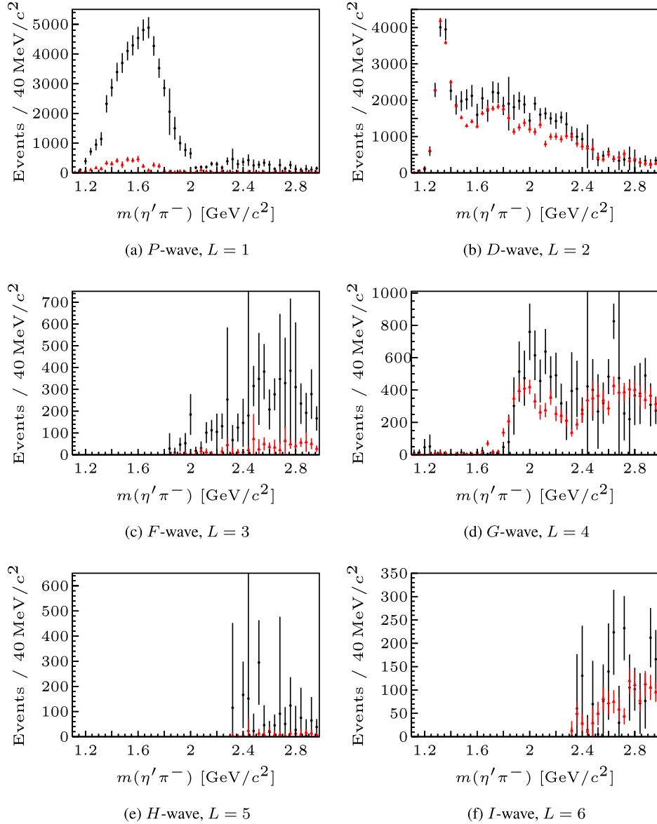
Fig. 4. Intensities of the L = 1-6 , M = 1 partial waves from the partial-wave analysis of the \eta'\pi^- data in mass bins of 40 \text{ MeV}/c^2 width (circles). Shown for comparison (triangles) are the \eta\pi^- results scaled by the relative kinematical factor given in Eq. (7).
