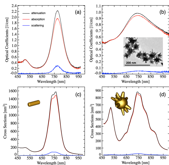
Figure 4. Top panel: Experimental attenuation (extinction), absorption, and scattering coefficients for nanorods (a) and nanostars (b). Inset shows a representative TEM image of nanostars. Relative absorption at the absorption maximum is 87.3% and 95.7% for nanorods and nanostars, respectively. Measurements were performed for different concentrations of nanorods and nanostars. Bottom panel: Theoretical extinction, absorption and scattering cross-sections for gold nanorods (c) and gold nanostars (d). All theoretical spectra were averaged over 100 random realizations of the corresponding geometries. Insets show representative examples of simulated structures. Relative absorption values at the absorption maxima are 94.5% and 97.1% for nanorods and nanostars, respectively.
