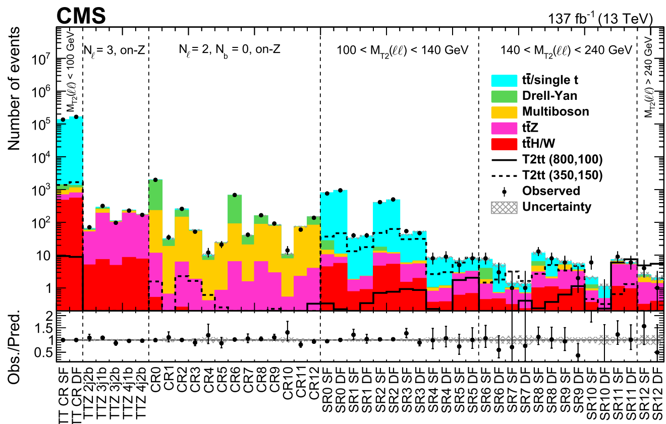
Fig. 5 Predicted and observed yields in the signal and control regions as defined in Tables 3 and 4. The control regions TTCSR and TTCSRDF are defined by M_{T2}(\ell\ell) < 100 GeV and are used to constrain the t\bar{t} normalization. The t\bar{t}Z control regions employ a 3 lepton requirement in different N_{\text{jets}} and N_b bins. The dilepton invariant mass and N_b selec-
