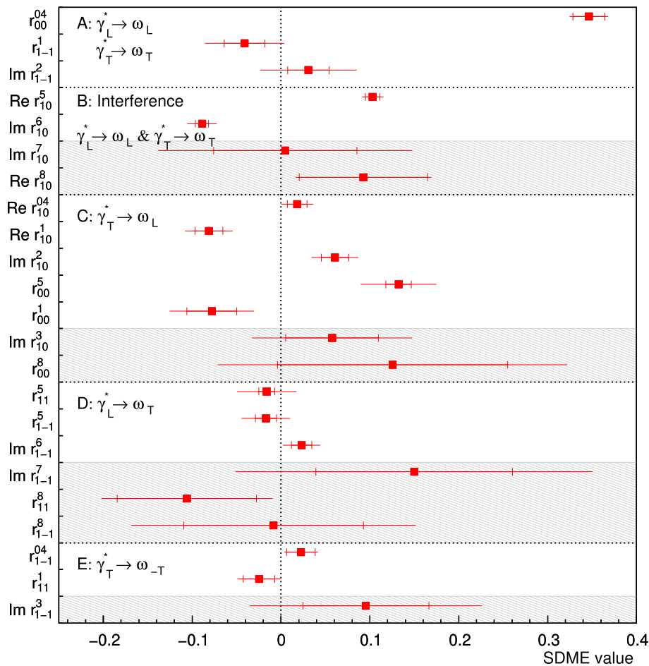
Fig. 5 The 23 SDMEs for exclusive \omega lepton production extracted in the total COMPASS kinematic region with \langle Q^2 \rangle = 2.13 \text{ (GeV}/c^2\text{)} , \langle W \rangle = 7.6 \text{ GeV}/c^2 , \langle p_T^2 \rangle = 0.16 \text{ (GeV}/c^2\text{)} . Inner error bars represent statistical uncertainties and outer ones statistical and systematic uncertainties added in quadrature. Unpolarised (polarised) SDMEs are displayed in unshaded (shaded) areas
