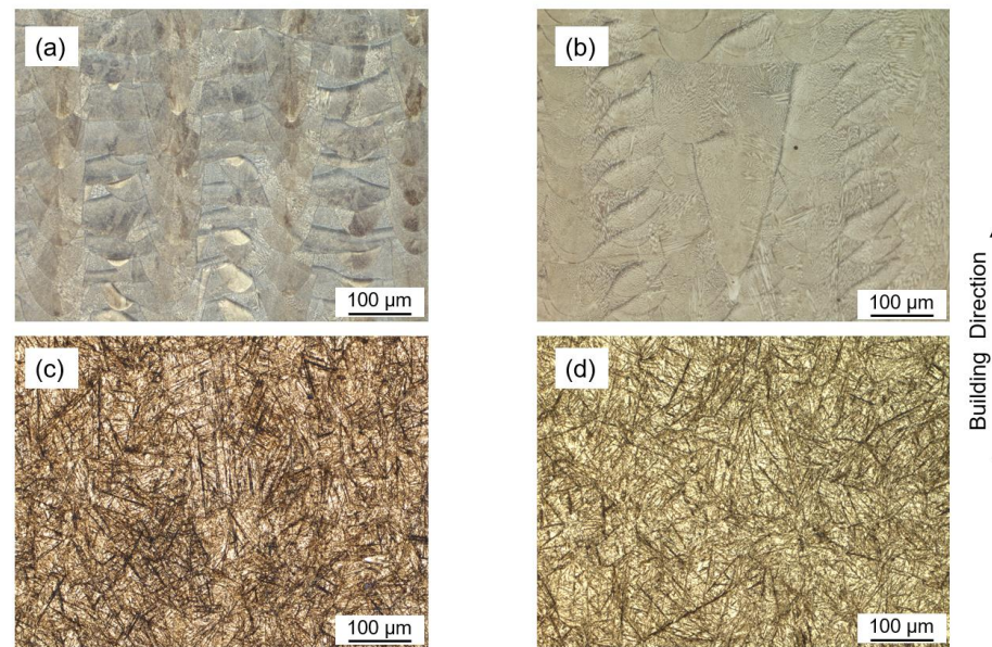
Figure 5. Optical micrographs: (a) as-built with a preheating of 250 °C; (b) as-built with a preheating of 500 °C; (c) conventional heat treatment; (d) HIP integrated with quenching and tempering.
