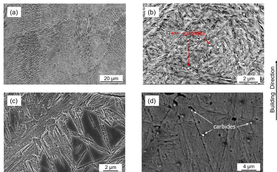
Figure 6. SEM images of microstructure. (a) as-built with 250 °C preheating; (b) conventional heat treatment; (c) HIP with quenching; (d) HIP with quenching and tempering.
