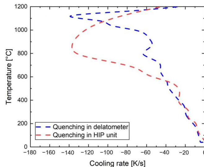
Figure 3. Cooling rate in dilatometer and HIP unit.
