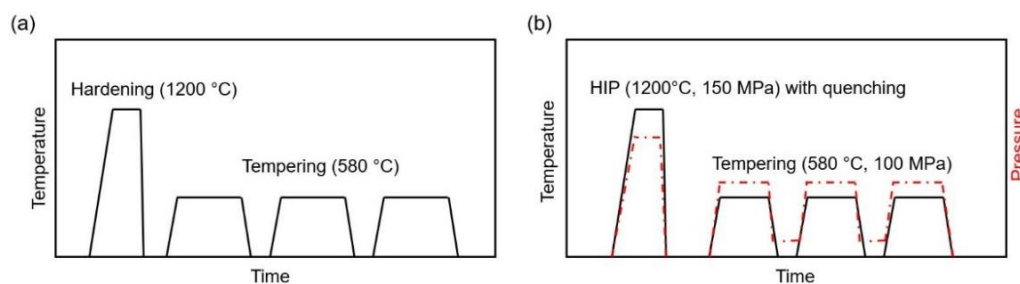
Figure 2. Schematic diagram of post treatments: (a) conventional heat treatment; (b) hot isostatic pressing (HIP) integrated with quenching and tempering.
