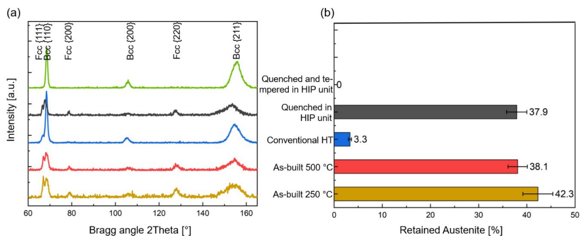
Figure 9. (a) XRD phase diffraction pattern and (b) retained austenite fraction in different conditions.
