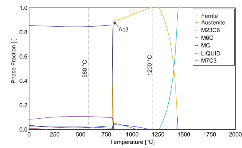
Figure 1. Calculated equilibrium phase fraction of the M50 powder.
