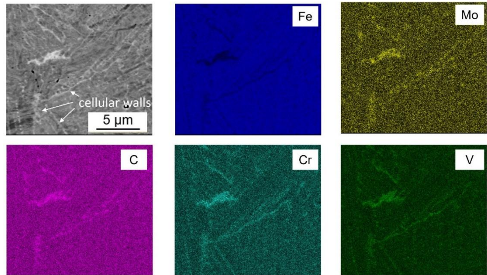
Figure 7. Backscattered-Electron (BSE) micrograph of the as-built sample with 250 °C preheating temperature and corresponding elemental Energy Dispersive Spectroscopy (EDS) mapping.
