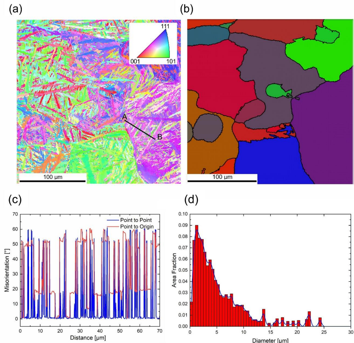
Figure 10. Microstructure analysis of the sample annealed and quenched in the HIP furnace. (a) An Inverse Pole Figure (IPF) map features the fine martensitic plates. (b) The corresponding parent austenite grains are reconstructed based on the EBSD result. (c) Point-to-point and point-to-origin misorientation profile of AB line in (a), which illustrates the width of martensite plates/blocks. (d) Martensitic plate width distribution.
