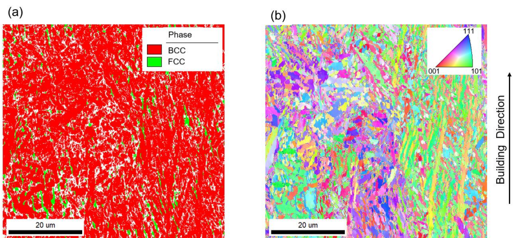
Figure 8. Electron Backscatter Diffraction (EBSD) phase map (a) and inverse pole figure map (b) of as-built sample produced at 250 °C.
