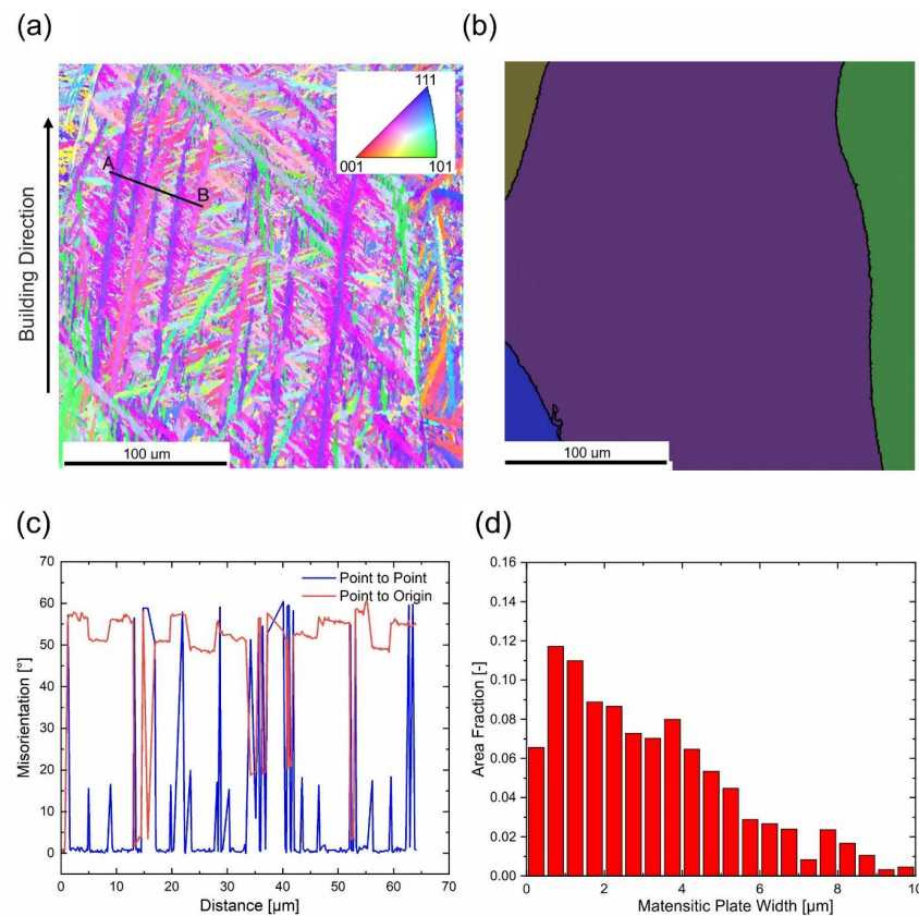
Figure 11. Microstructure analysis of the sample annealed and quenched in dilatometer. (a) Relative coarse martensite is presented by the IPF map. (b) The corresponding parent austenite is reconstructed based on EBSD result. (c) Point-to-point and point-to-origin misorientation profile of AB line in (a). (d) Martensitic plate width distribution.
