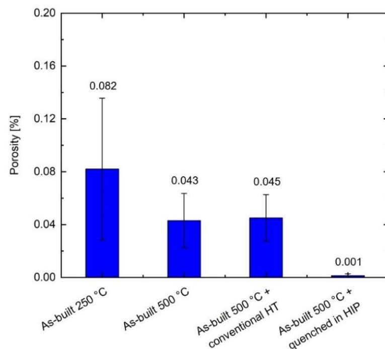
Figure 4. Porosity (middle value and standard deviation) in different conditions. For the two post treatments, samples built with preheating at 500 °C were used.
