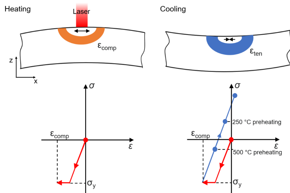
Figure 13. Schematic illustration of temperature gradient mechanism (TGM) model, according to [6].
