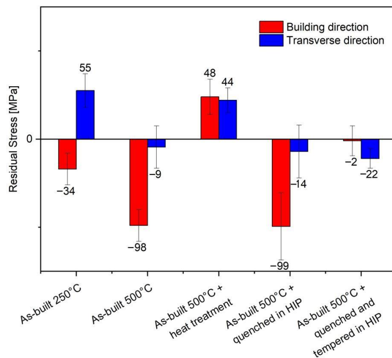
Figure 12. Residual stresses in different conditions.
