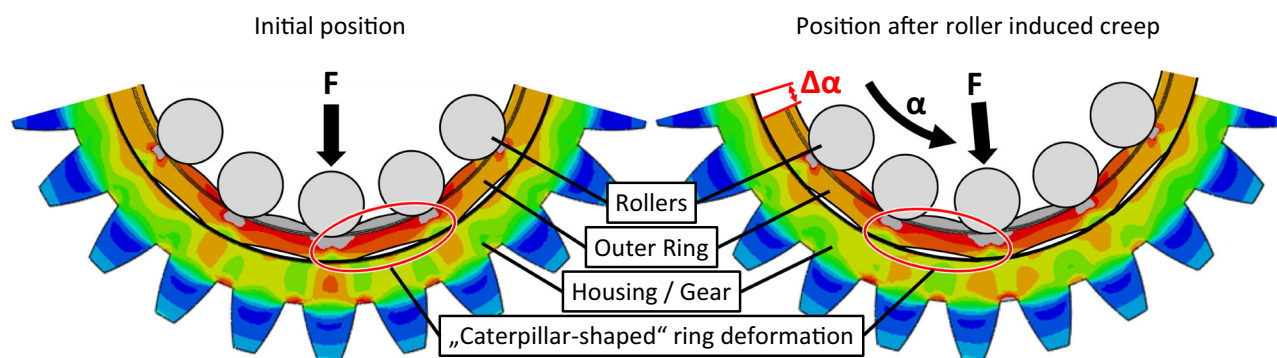
Fig. 1 Schematic model of roller-induced ring creep and the “caterpillar-shaped” deformation (exaggerated) of the bearing ring [5]
