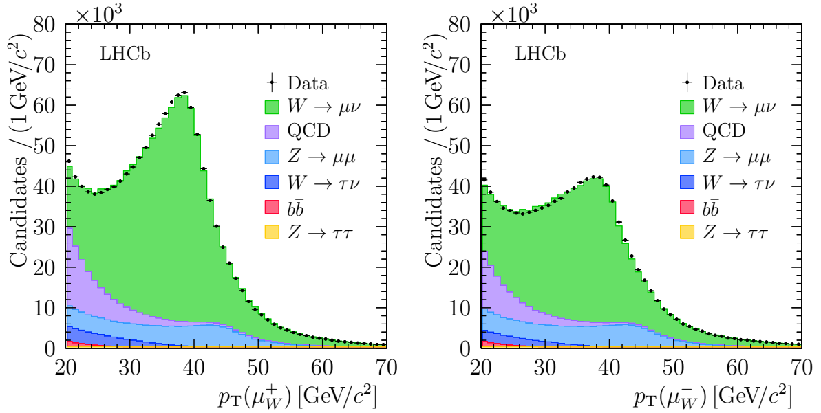
Figure 3: The (left) positive and (right) negative muon transverse momentum spectra for the 2012 data set integrated over pseudorapidity for the normalisation channel. The filled histograms are the result of the fit to the data.
