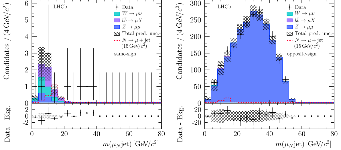
Figure 4: Distributions of the invariant mass m(\mu_N \text{ jet}) for (left) same-sign and (right) opposite-sign muons. The signal component corresponds to a 15 \text{ GeV}/c^2 neutrino.
