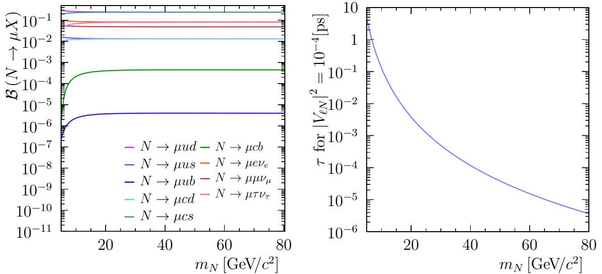
Figure 1: Properties of a heavy neutrino as a function of its mass [21,22]: (left) the branching fractions to final states with a muon and (right) the lifetime, assuming a coupling of 10^{-4} .
