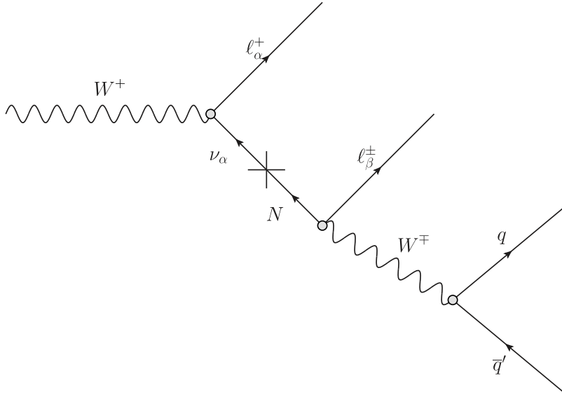
Figure 2: Feynman diagram for the production of a heavy neutrino via mixing with a neutrino from the decay of a W boson and semileptonic decay of the heavy neutrino into a lepton and two quarks. The subscripts \alpha and \beta indicate the lepton flavour. In this analysis \alpha and \beta are both muons.
