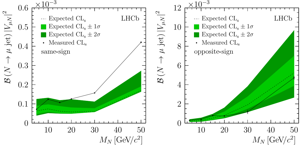
Figure 5: Expected (dashed line) and observed (solid line) upper limit on \mathcal{B}(N \rightarrow \mu \text{ jet}) |V_{\mu N}|^2 at 95% C.L. for (left) the same-sign muons sample and (right) the opposite-sign muons sample. The light and dark green bands show the 1\sigma and 2\sigma uncertainties, respectively, on the expected upper limits.
