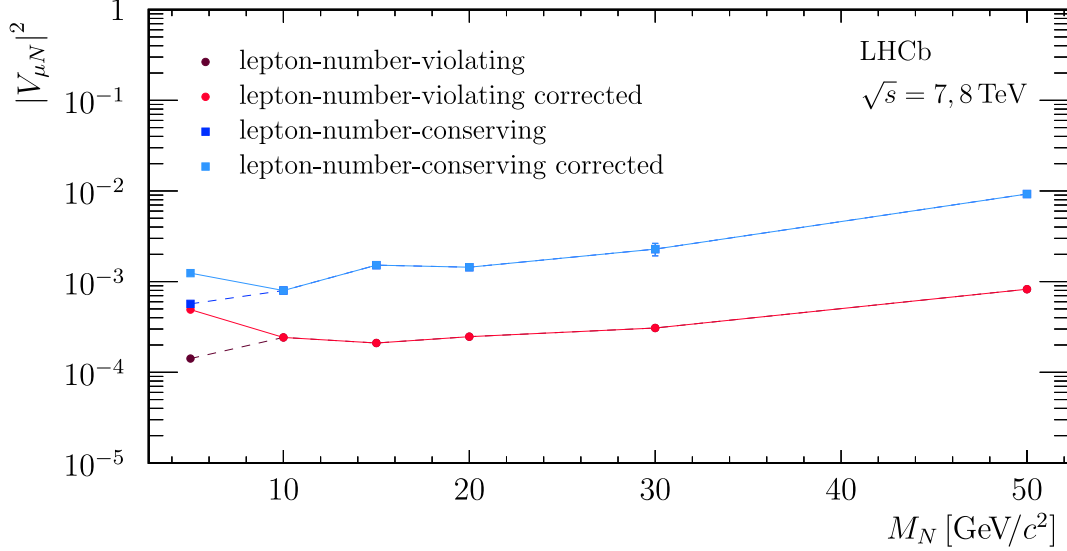
Figure 6: Observed upper limit on the mixing parameter |V_{\mu N}|^2 between a heavy neutrino and a muon neutrino in the mass range 5 – 50 GeV/ c^2 for same-sign and opposite-sign muons in the final states with and without lifetime correction.
