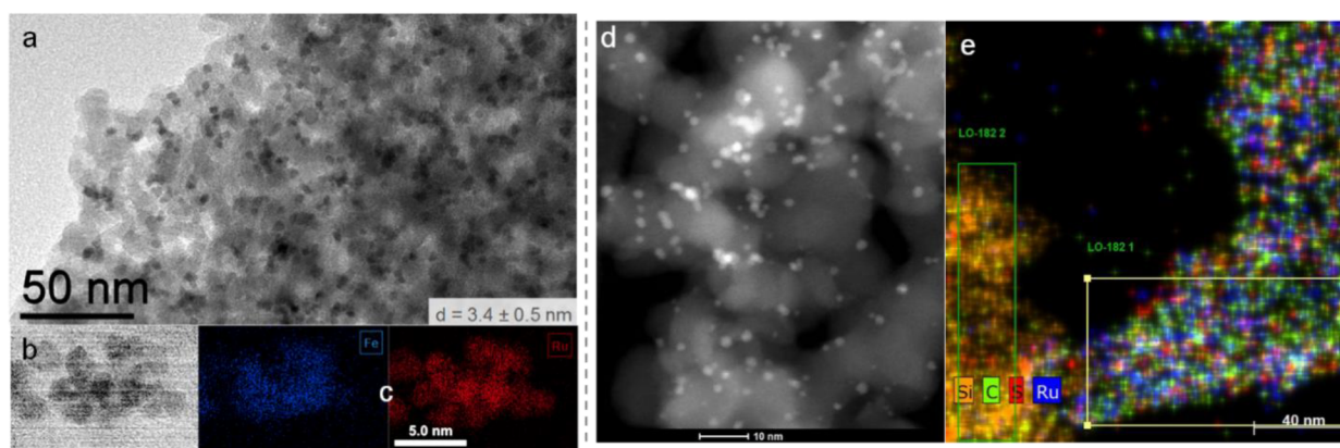
Figure 4. Characterization of NPs@MMS materials using electron microscopy. Left: \text{Fe}_{25}\text{Ru}_{75}\text{@SILP} catalyst 31 characterized by (a) TEM; (b) STEM; (c) STEM-HAADF-EDX with elemental mapping. Right: \text{Ru@SILP-SO}_3\text{H} catalyst 23 characterized by (d) STEM-HAADF; (e) STEM-HAADF-EDX with elemental mapping.
