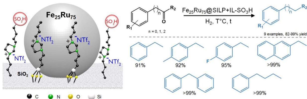
Figure 12. Selective hydrodeoxygenation of benzylic and nonbenzylic ketones using a \text{Fe}_{25}\text{Ru}_{75} @SILP+IL- \text{SO}_3\text{H} catalyst.
