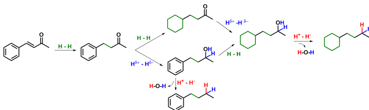
Figure 5. Reaction pathway for the hydrogenation and hydrodeoxygenation of benzylideneacetone, evidencing the H 2 activation requirements for each transformation.
