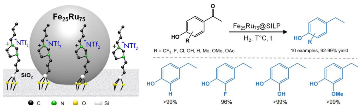
Figure 13. Selective hydrodeoxygenation of hydroxyacetophenone derivatives using a \text{Fe}_{25}\text{Ru}_{75} @SILP catalyst.
