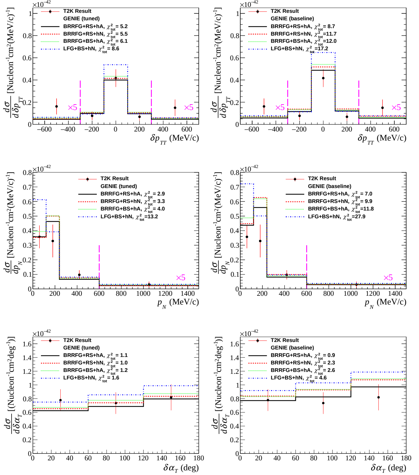
FIG. 15. Measured differential cross sections per nucleon as a function of \delta p_{TT} (top), p_N (middle) and \delta \alpha_T (bottom), together with predictions from the different model configurations of GENIE. The left plots use the free nucleon cross section re-tune, and the right plots use the baseline tune. In the tails of \delta p_{TT} and p_N (beyond the magenta lines), the cross sections are scaled by a factor of 5 for better visualization. The legend also shows the \chi^2_{\text{tot}} from Eq. (17).
