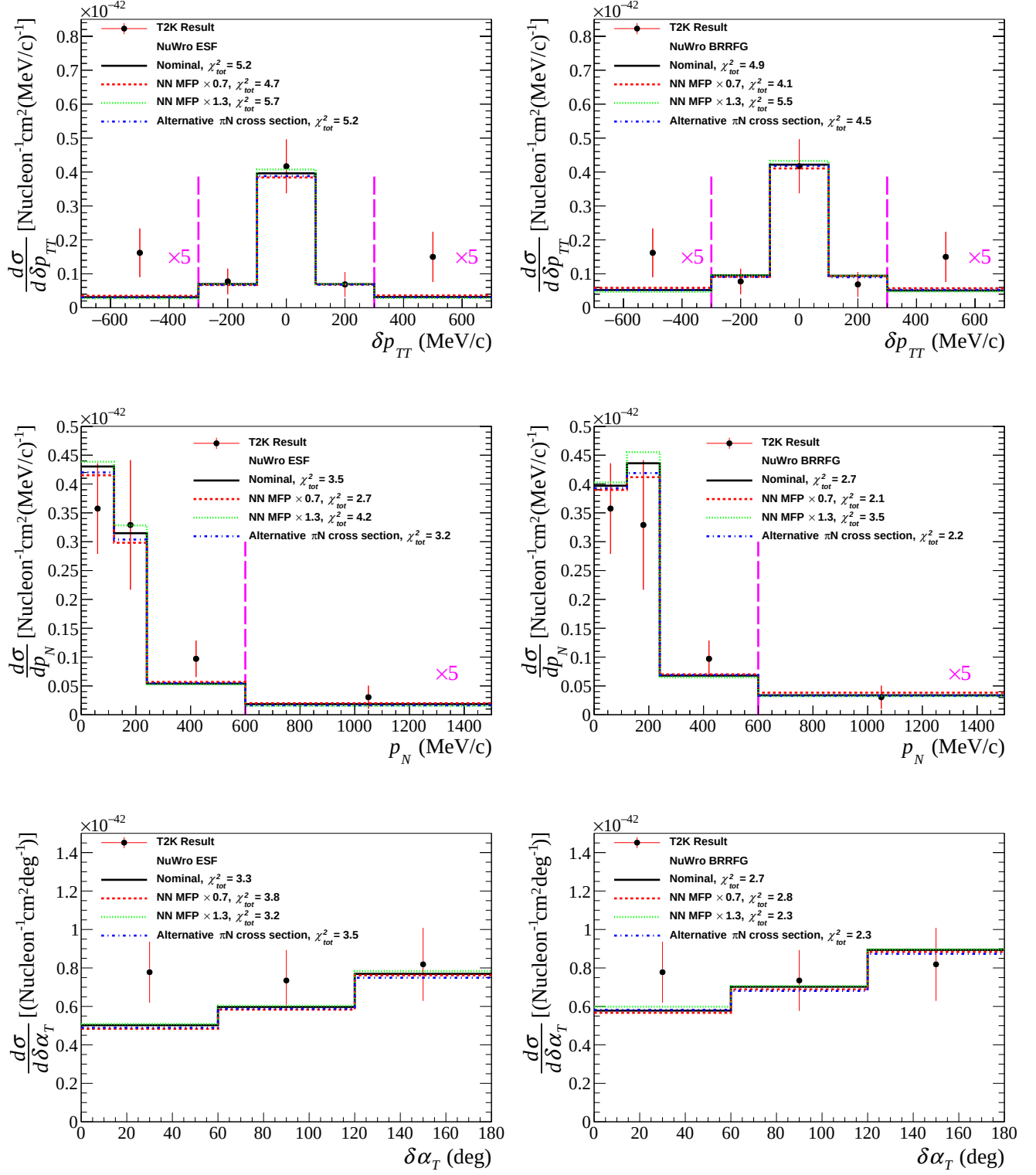
FIG. 16. Measured differential cross sections per nucleon as a function of \delta p_{TT} (top), p_N (middle) and \delta \alpha_T (bottom), together with predictions from the NuWro ESF (left) and BRRFG (right) models. The black solid line shows the prediction from the nominal FSI configuration, while other colors show that from a different nucleon mean free path (NN MFP) or pion-nucleon ( \pi N ) interaction model configuration. In the tails of \delta p_{TT} and p_N (beyond the magenta lines), the cross sections are scaled by a factor of 5 for better visualization. The legend also shows the \chi^2_{\text{tot}} from Eq. (17).
