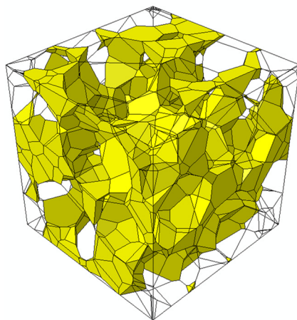
Figure 6. The generated RVEs (with sizes of 10\ \mu\text{m} \times 10\ \mu\text{m} \times 10\ \mu\text{m} ) for each investigated steel. The grains and number of grains for each phase are shown.
