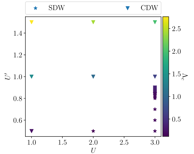
FIG. 8. Phase diagram of the vertex Penrose model employing Eq. (C2). We find a SDW (star marker) and a CDW (triangular marker) phase. The critical scales are given by the color code.
