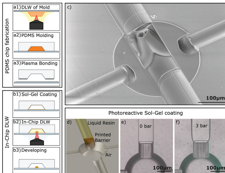
Figure 1. The fabrication process of the microfluidic device consisting of the PDMS chip fabrication (a) and in-chip DLW (b). The PDMS chip fabrication includes direct laser writing of the mold (a1), the PDMS molding (a2), and the plasma bonding of the PDMS chip to a glass slide (a3). The in-chip direct laser writing process includes the sol-gel coating for increased adhesion (b1), the in-chip direct laser writing (b2), and the development of the device (b3). The scanning electron microscopy (SEM) image of the imprinted three-fluid contactor nozzle has a custom 3D-geometry for versatile spinning applications of one and two fluids (c). The photoreactive sol-gel coating (b1) was tested in a burst pressure experiment (d) by applying 0 bar (e) and 3 bar (f) trans-barrier pressure to an imprinted 10 \mu\text{m} thick barrier.
