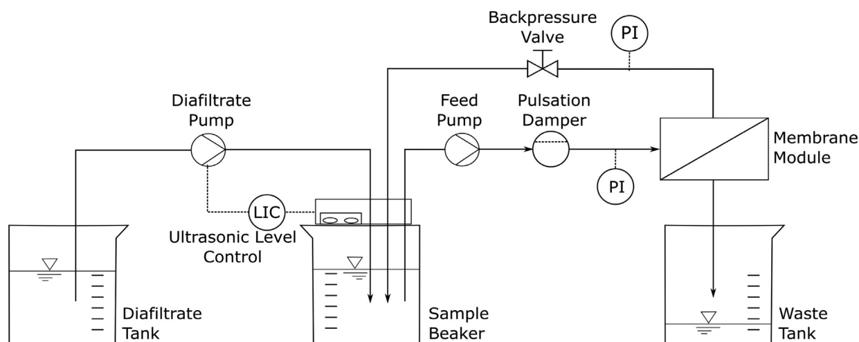
Fig. 1. Piping and instrument drawing of the filtration process.
