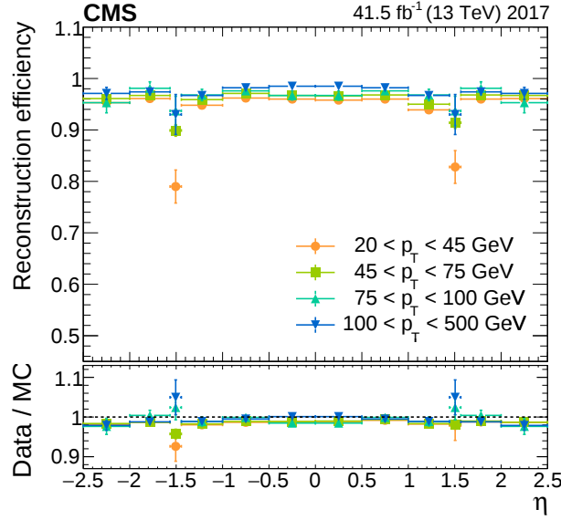
Figure 4: Electron reconstruction efficiency versus \eta in data (upper panel) and data-to-simulation efficiency ratios (lower panel) for the 2017 data taking period. The vertical bars on the markers represent the combined statistical and systematic uncertainties. The region 1.44 < |\eta| < 1.57 corresponds to the transition between the barrel and endcap regions of ECAL and is not considered in physics analyses.
