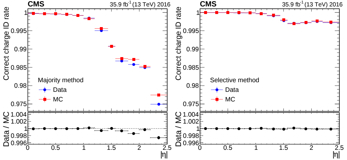
Figure 7: Correct charge identification probability for electrons using the majority method (left) and the selective method (right), as measured in the 2016 data set and in simulated Z \rightarrow e\bar{e} events. The electrons are required to satisfy the loose identification requirements described in Section 7.3. The uncertainties assigned to the points are statistical only.
