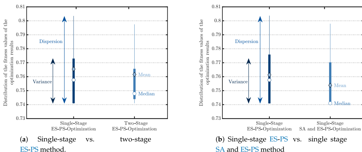
Figure 5. Comparison of the distribution of results for different optimization methods.
