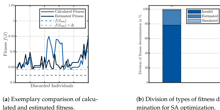
Figure 6. Exemplary comparison of calculated and estimated fitness (a) and the breakdown of fitness determination (b).
