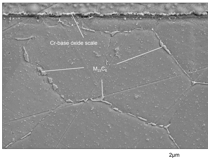
Figure 15.21: SEM image of the cross section of 1.4910 after 1000h exposure to Ar/CO 2 at 650°C
