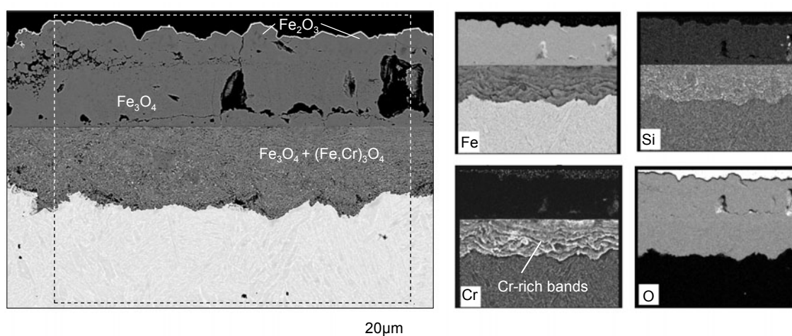
Figure 13.6: SEM image of the cross section of P92 after 1000h oxidation in Ar/CO 2 at 650°C and corresponding X-ray element mappings from the marked area
