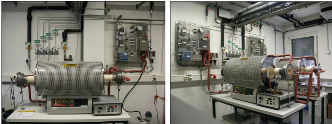
Figure 4.3: Horizontal experimental set-up for long- and short-term exposures in mixed gas environments
