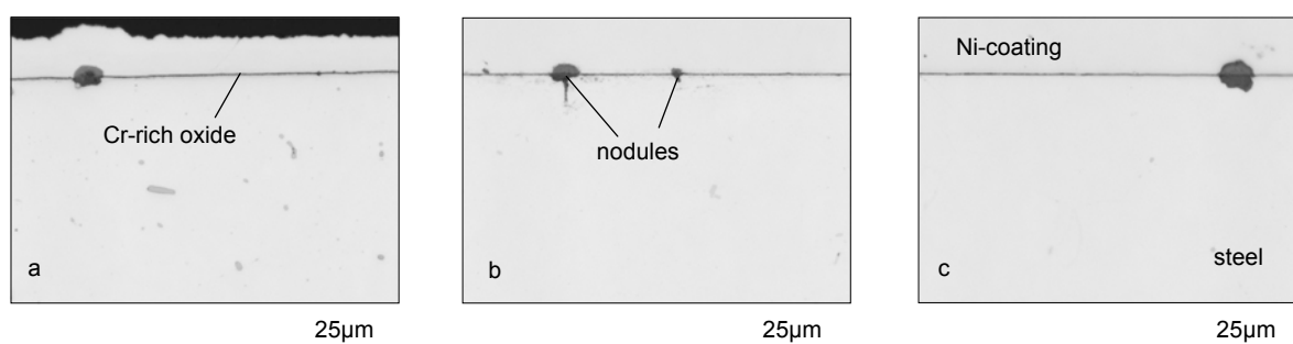
Figure 6.6: Metallographic cross sections of TP347H FG (a); Super 304H (b) and 310N (c) oxidized in Ar/CO 2 for 1000h at 550°C
