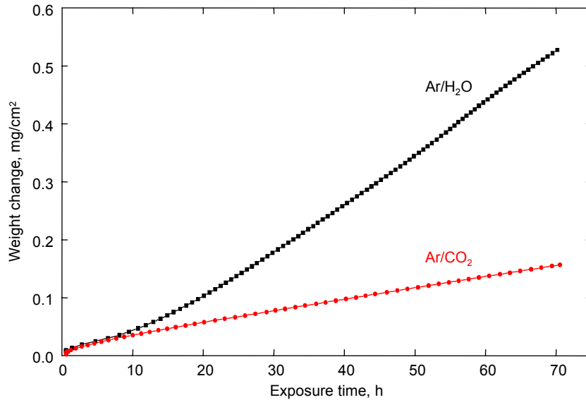
Figure 12.2: Thermogravimetric curves of P92 during isothermal oxidation in \text{Ar}/(2\%)\text{CO}_2 and \text{Ar}/(2\%)\text{H}_2\text{O} at 550^\circ\text{C}
