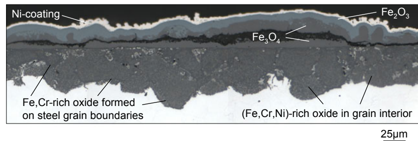
Figure 6.18: Metallographic cross section of 1.4910 after 1000h exposure to CO 2 /H 2 O at 700°C
