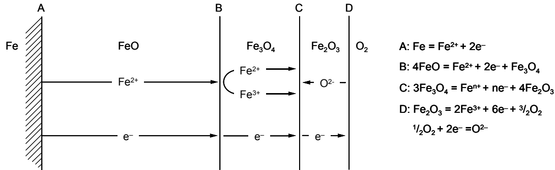
Figure 3.6: Schematic illustration of the oxide layers formed during iron oxidation above 570°C in a high \text{pO}_2 gas and the dominant diffusing species through each oxide layer. The reactions that take place at each interface are presented on the right side. Based on [20, 32]
