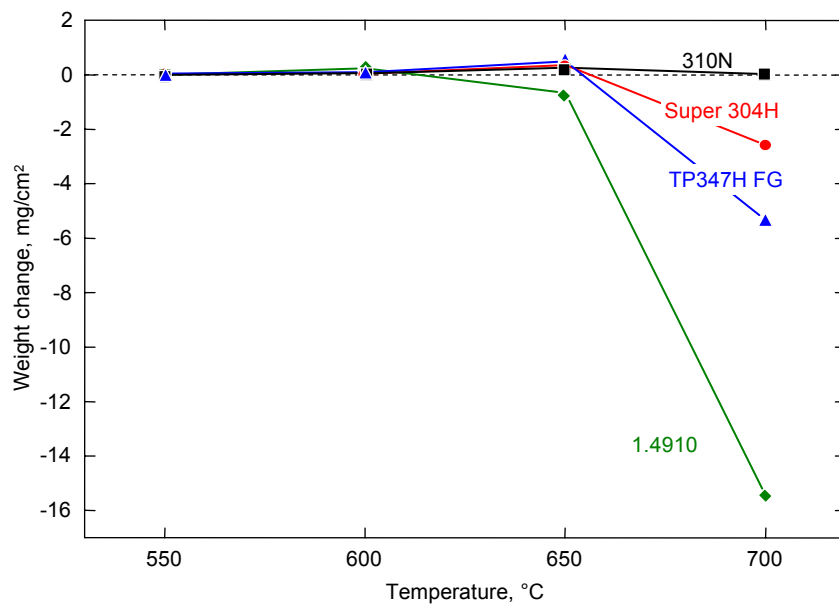
Figure 6.13: Weight changes of austenitic steels after 1000h oxidation in Ar/CO 2 at 550-700°C
