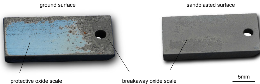
Figure 14.7: Macroscopic pictures of ground (left) and sandblasted (right) VM12 specimens after 1000h exposure to Ar/O 2 /CO 2 /H 2 O at 600°C
