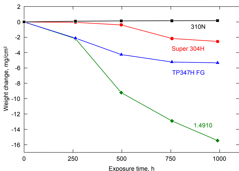
Figure 6.11: Weight changes of austenitic steels during oxidation in Ar/CO 2 at 700°C
