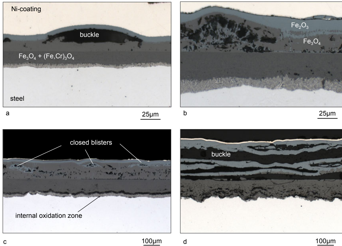
Figure 5.25: Metallographic cross sections of P92 after 1000h oxidation in Ar/O 2 /CO 2 /H 2 O at: 550°C (a); 600°C (b); 650°C (c) and 700°C (d)
