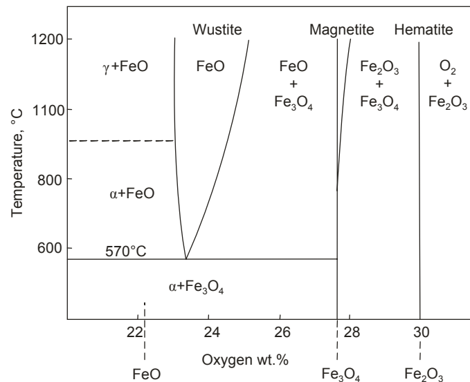
Figure 8.11: Part of iron-oxygen phase diagram. Reproduced from [26]
