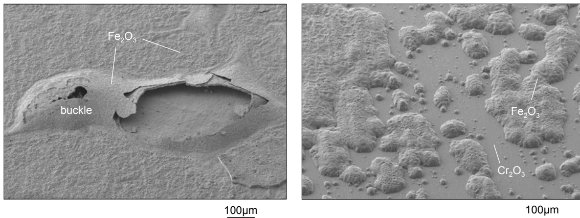
Figure 5.18: SEM images of the oxide surface formed on the P92 (left) and VM12 (right) after 1000h exposure to \text{CO}_2/\text{H}_2\text{O} at 550°C
