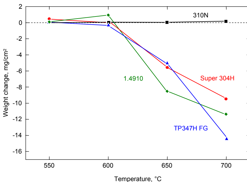
Figure 6.17: Weight changes of austenitic steels after 1000h exposure to \text{CO}_2/\text{H}_2\text{O} at 550\text{--}700^\circ\text{C}
