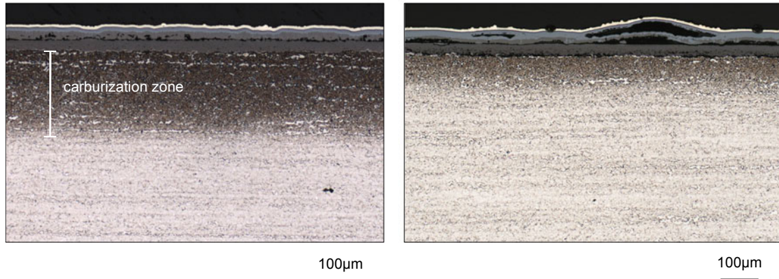
Figure 15.13: Etched cross sections of HCM12 after 1000h exposure in Ar/CO 2 (left) and CO 2 /H 2 O (right) at 600°C
