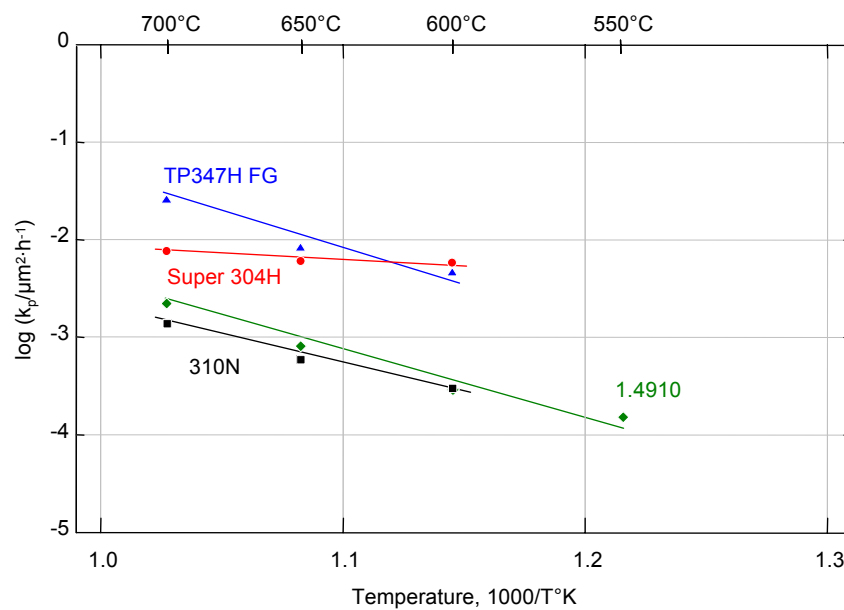
Figure 6.1: Parabolic rate constants as a function of reciprocal temperature of austenitic steels oxidized in laboratory air ( k_p derived from scale thickness measurements)
