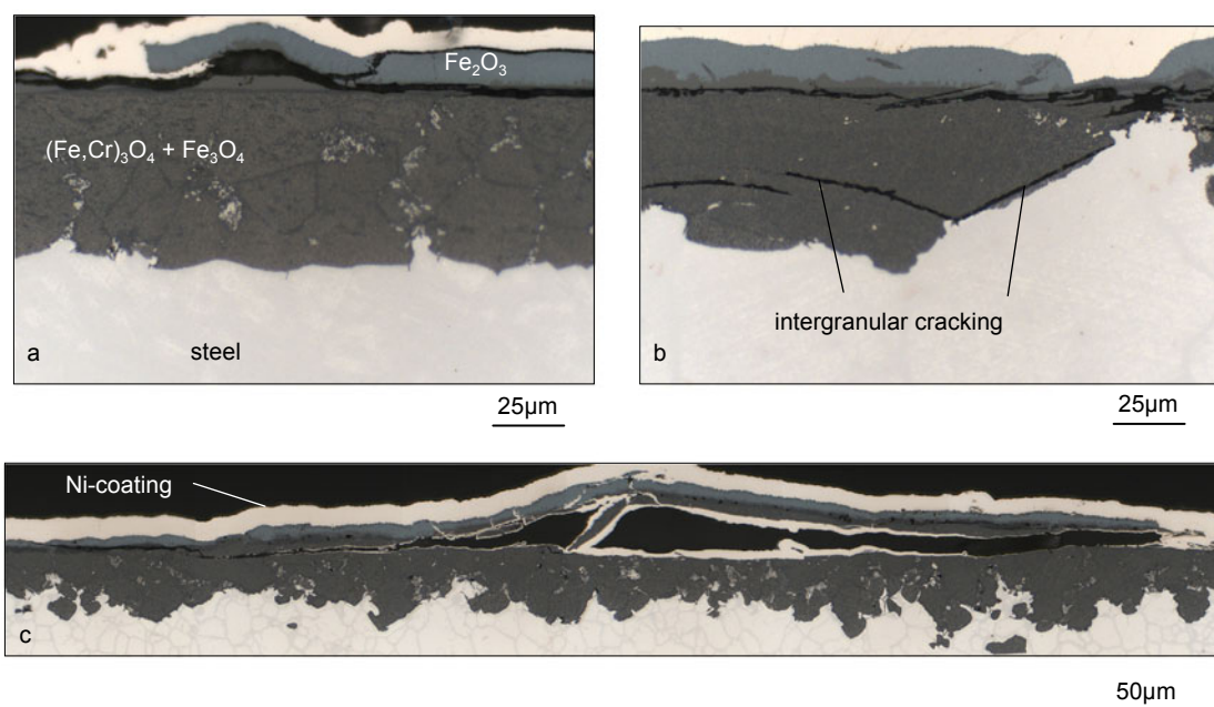
Figure 6.16: Metallographic cross sections of 1.4910 (a); TP347H FG (b) and Super 304H (c) after 1000h exposure to \text{CO}_2/\text{H}_2\text{O} at 650^\circ\text{C}
