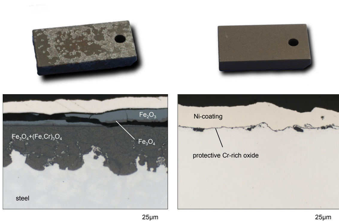
Figure 14.11: Macro images and cross sections of ground (left) and sandblasted (right) 1.4910 specimens after 1000h exposure to Ar/O 2 /CO 2 /H 2 O at 650°C
