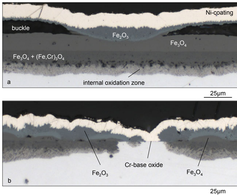
Figure 5.19: Metallographic cross sections of P92 (a) and VM12 (b) after 1000h oxidation in \text{CO}_2/\text{H}_2\text{O} at 550°C
