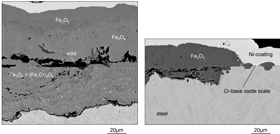
Figure 5.14: SEM images of the cross section of P92 (left) and VM12 (right) oxidized in Ar/CO 2 for 1000h at 700°C
