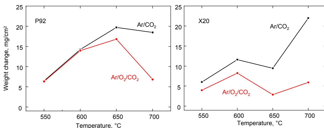
Figure 10.5: Temperature dependence on weight change for P92 (left) and X20 (right) after 1000h exposure to Ar/CO 2 (black) and Ar/(1%)O 2 /CO 2 (red)
