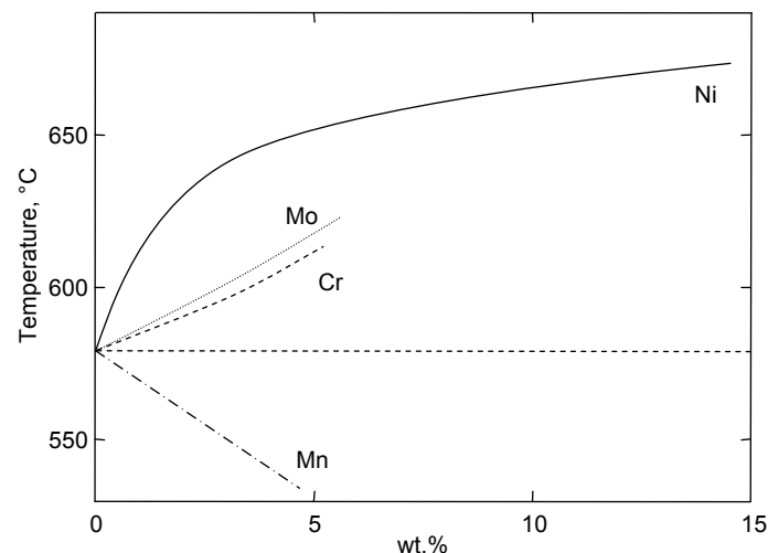
Figure 8.12: Effect of alloying elements on the temperature of wustite occurrence in the scale during oxidation in air. Reproduced from [103]
