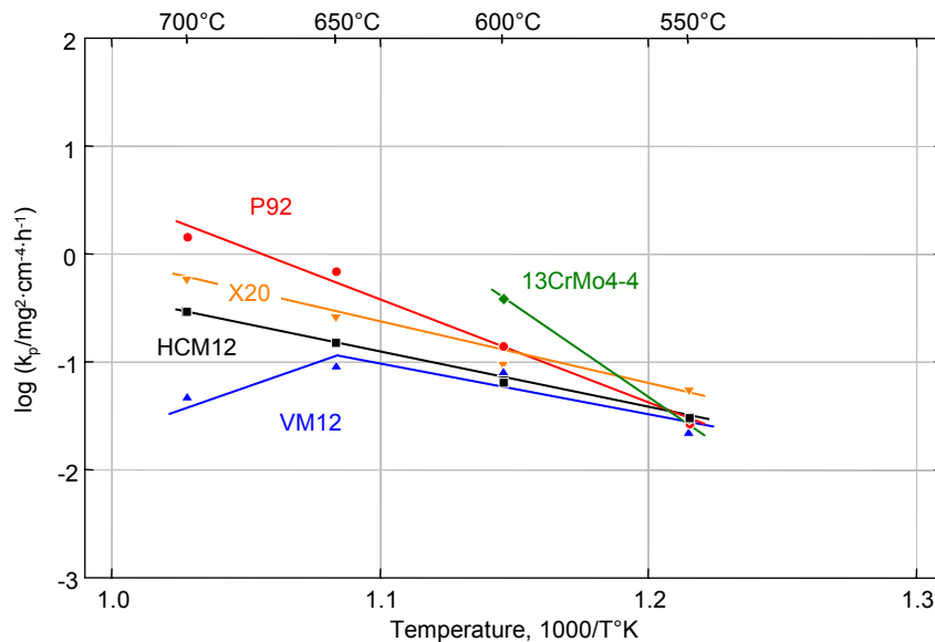
Figure 5.16: Parabolic rate constants as a function of reciprocal temperature of selected steels oxidized in CO 2 /H 2 O ( k_p derived from the weight change measurements)
