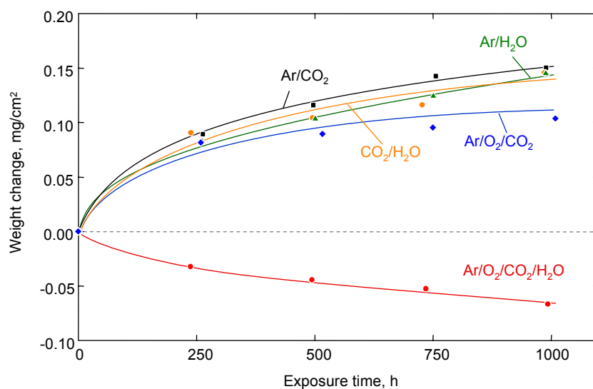
Figure 11.7: Weight changes of INCONEL 617 during 1000h exposure to different atmospheres at 700°C
