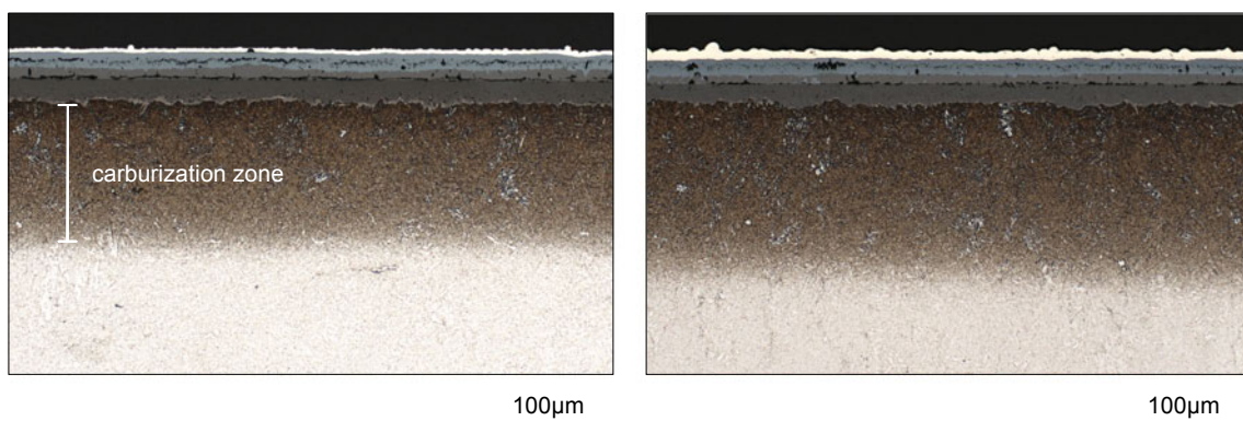
Figure 15.18: Etched cross sections of VM12 after 1000h exposure to Ar/CO 2 (left) and Ar/O 2 /CO 2 (right) at 600°C
