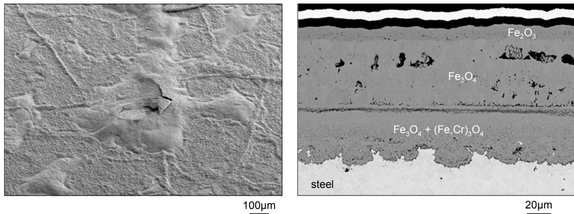
Figure 5.6: SEM images of the oxide surface (left) and cross section (right) of 13CrMo4-4 oxidized in Ar/H 2 O for 1000h at 600°C
