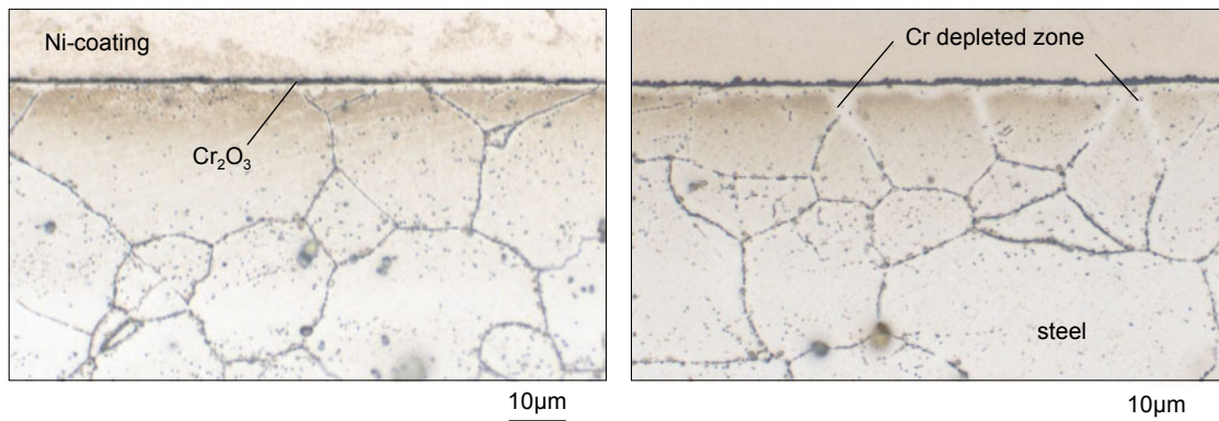
Figure 6.19: Metallographic cross sections of 310N after 1000h exposure to CO 2 /H 2 O at 650°C (left) and 700°C (right). Cross sections etched in NH 3 solution
