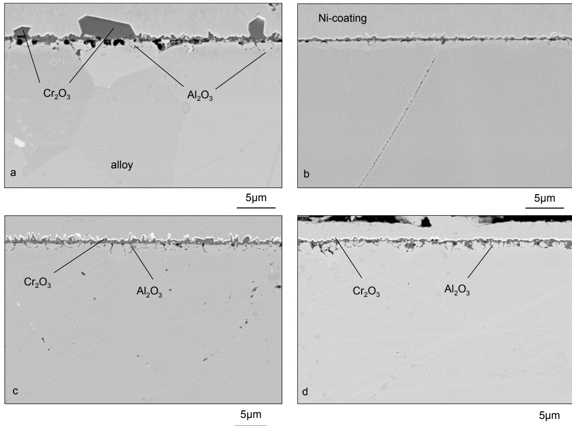
Figure 7.2: SEM images of the cross sections of INCONEL 617 after 1000h oxidation in laboratory air (a); Ar/CO 2 (b); CO 2 /H 2 O (c) and Ar/O 2 /CO 2 /H 2 O (d) at 700°C
