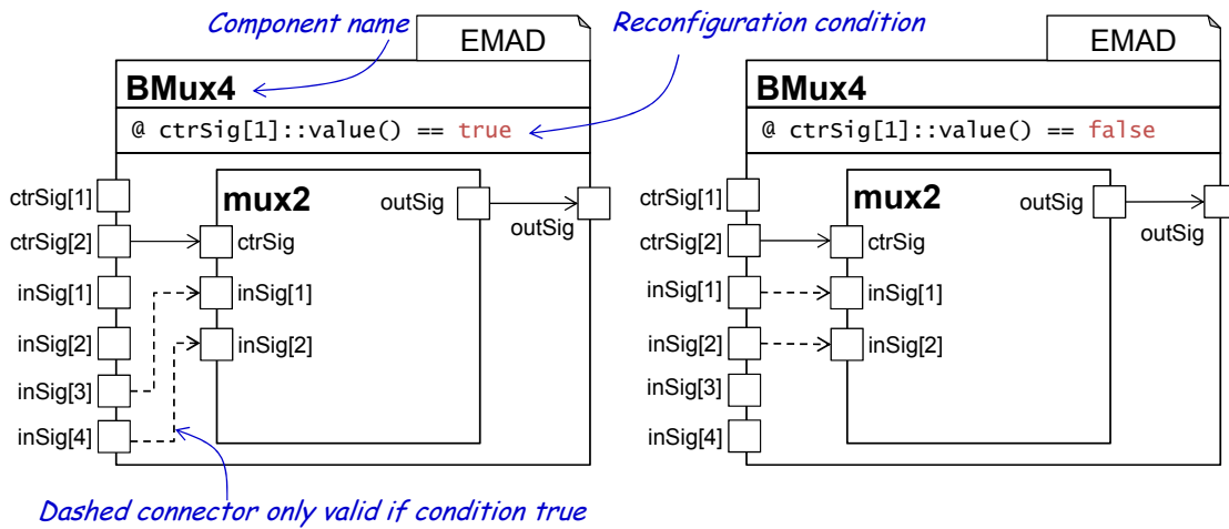
Figure 3.2: The two architectural states of the BMux4 component.
