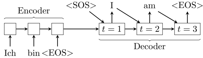
Figure 4.19: RNN encoder-decoder model example [KNP + 19].
