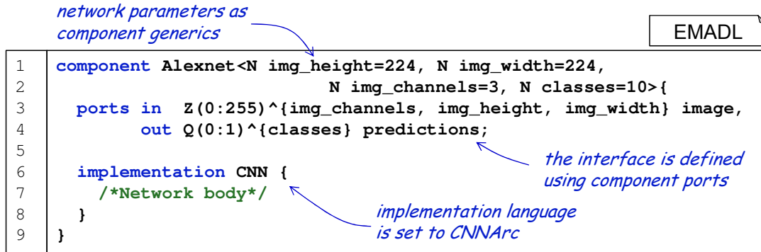
Figure 4.23: Definition of an EMADL component with a MontiAnna neural network implementation.
