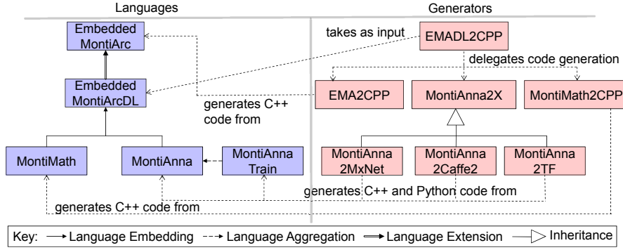
Figure 4.22: An overview of the EmbeddedMontiArcDL modeling language family: languages and code generators are depicted as purple and pink boxes, respectively [KPRS19].
