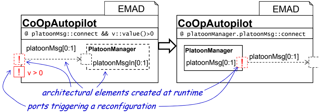
Figure 3.11: A reconfiguration chain involving input and output ports of the PlatoonManager component. An arriving platoon message causes the creation of new input ports in the diagram on the left. Follow-up reconfigurations inside the PlatoonManager result in a new output port and a new outgoing connector as depicted in the diagram on the right.
