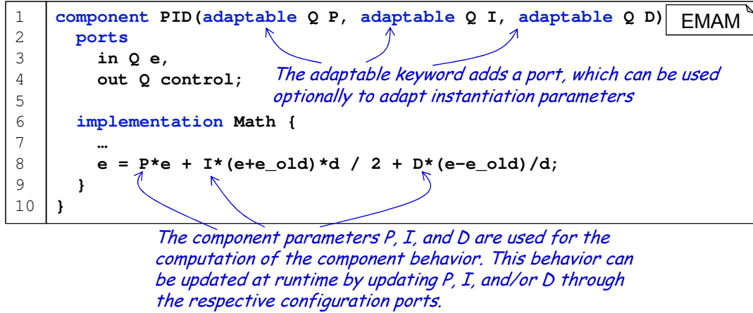
Figure 2.17: The PID component interface with adaptable parameters defined in EmbeddedMontiArc.
