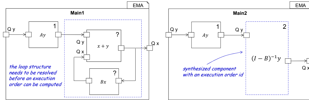
Figure 2.8: This example shows an architecture featuring an algebraic loop (Main1) and its loop-free equivalent synthesized automatically at compile-time (Main2).
