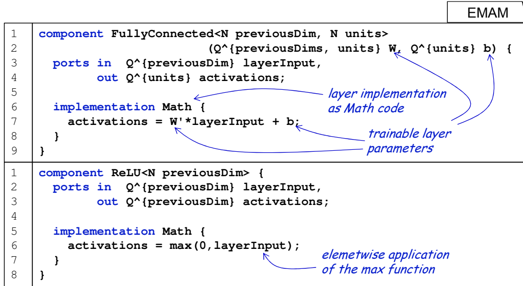
Figure 4.18: An example showing how MontiMath could be used to implement custom layers for MontiAnna networks.
