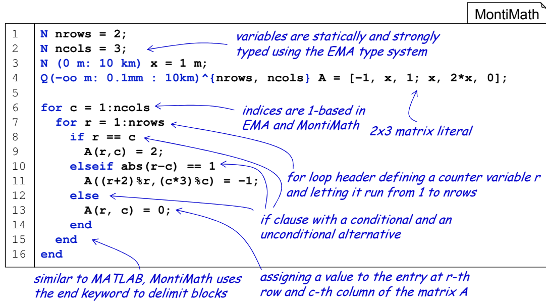
Figure 2.10: This listing shows a simple MontiMath example exhibiting the main language constructs including variable declarations, matrix literal definitions, loops and if statements.
