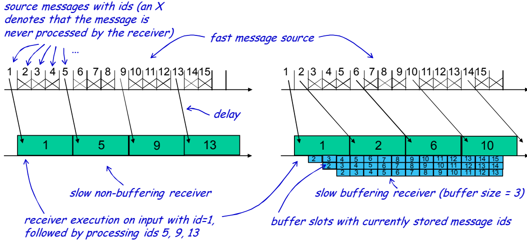
Figure 6.9: Setting in which a fast sender serves a slow receiver with and without buffering.
