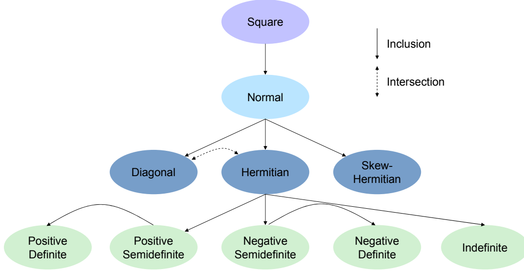
Figure 2.1: A simplified taxonomy of matrices containing the matrix properties relevant for the EMA type system based on [HJ90].
