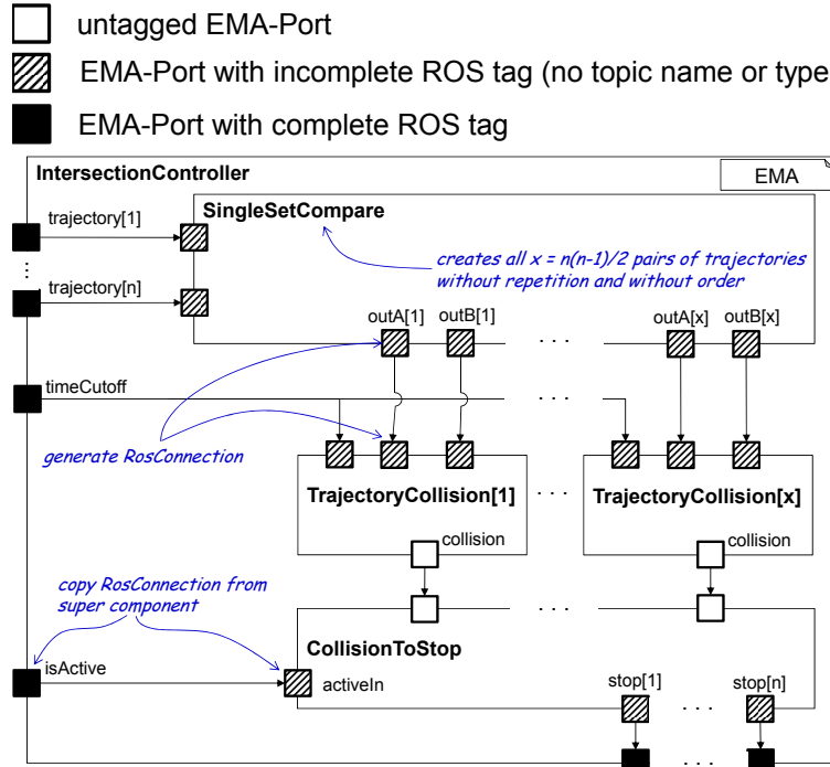
Figure 6.2: Intersection controller model with middleware tags attached to its ports [HKKR19].
