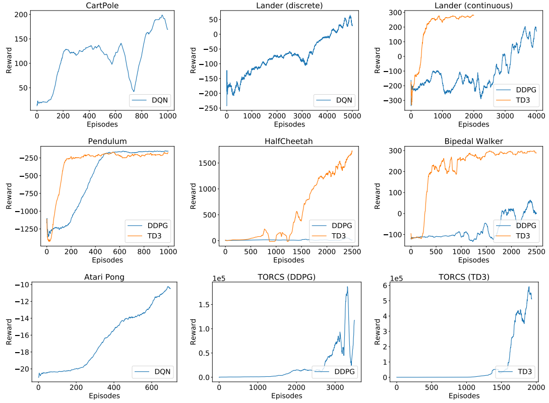
Figure B.1: The average reward over the last 100 episodes during training for OpenAI Gym and TORCS experiments using MontiAnna models conducted by Nicola Gatto in his master's thesis.
