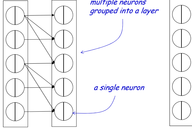
Figure 4.2: The abstraction of layers in artificial neural networks.
