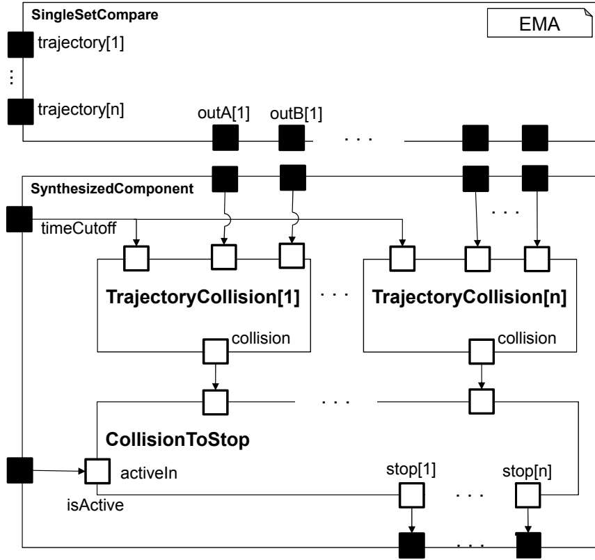
Figure 6.6: True deployment scheme of the intersection controller with two separately deployable components.
