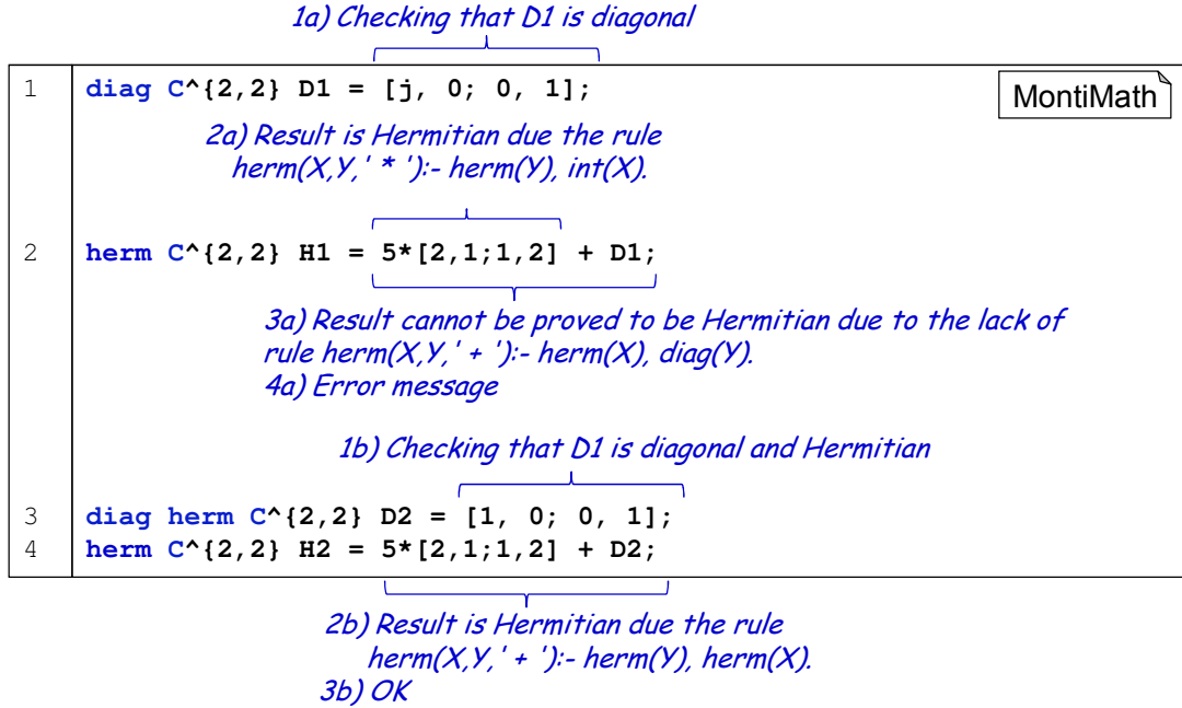
Figure 2.12: An example of matrix property derivation for operations.
