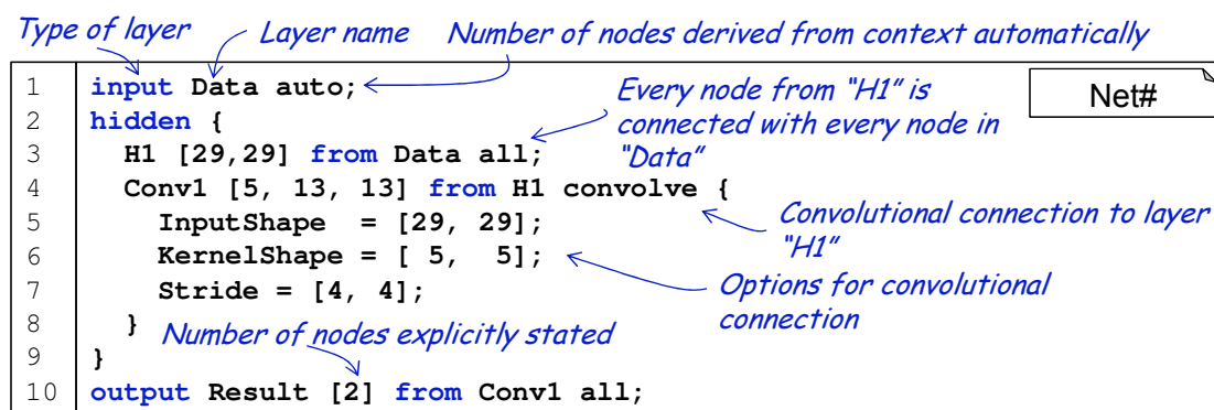
Figure 4.5: Neural network architecture defined in Net# [KPRS19].
