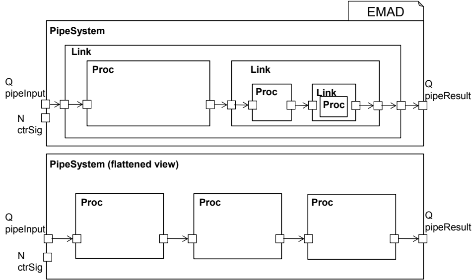
Figure 3.7: The pipe system component on top shows the structure of an arbitrarily long pipeline as defined in Figure 3.8. The last (or deepest) link component contains only a processing but no more linking subcomponents. Since EMA flattens hierarchical components, the effective architecture is a simple pipeline as shown in the bottom model.
