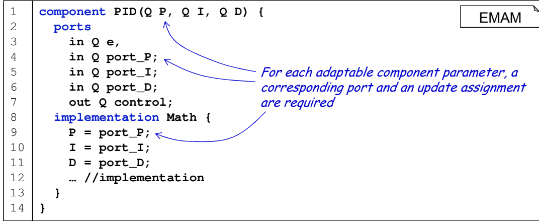
Figure 2.16: The PID component with parameters adaptable through dedicated ports.
