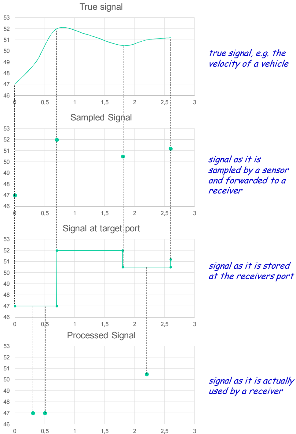
Figure 6.10: The four plots show an exemplary propagation of a signal through a middleware-based EMA component network.
