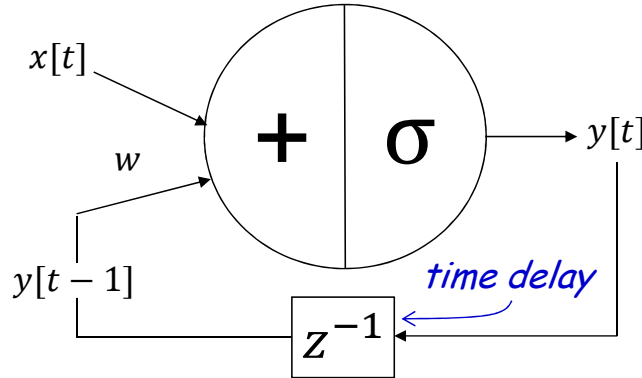
Figure 4.3: The vanilla RNN cell model.
