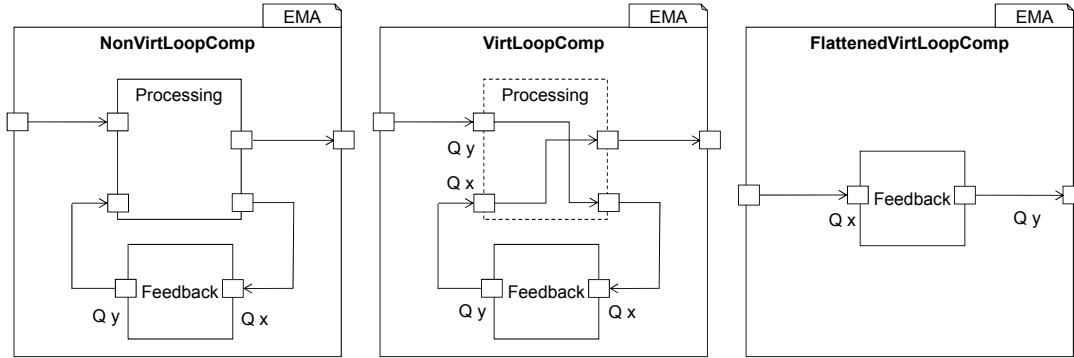
Figure 2.9: The component on the left contains a loop consisting of two non-flattened components. The model in the middle displays the contents of the Processing subcomponent making obvious that there are no circular dependencies on port level. The figure on the right shows how the component is seen by the compiler after the flattening step.
