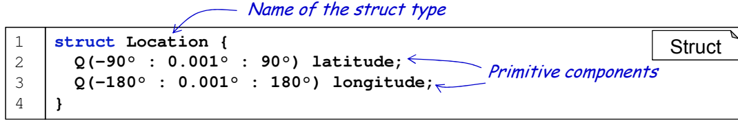
Figure 2.2: A struct example encapsulating the primitive variables longitude and latitude into a type named Location.
