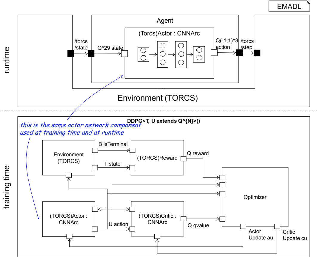
Figure 5.6: The upper part of the figure depicts the top level runtime C&C model of the DDPG-based TORCS controller. The filled ports highlight the reinforcement learning interface. The connections between them are generated based on the middleware tagging approach, which will be presented in Chapter 6. The training reference architecture of the DDPG algorithm is depicted in the bottom part and contains a critic, a reward, an environment, and a trainer component, which are thrown away at runtime.
