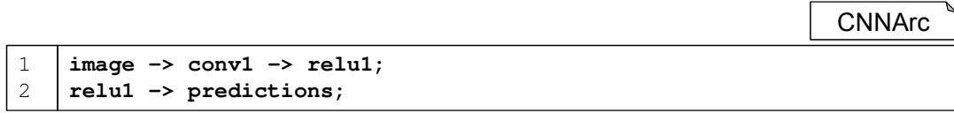
Figure 4.10: A neural network represented as two graph expressions.
