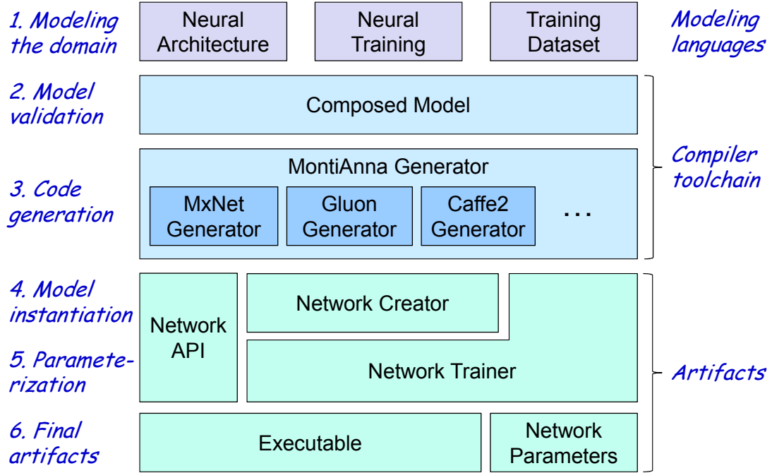
Figure 4.6: Overview of the MontiAnna framework layers [KNP + 19].
