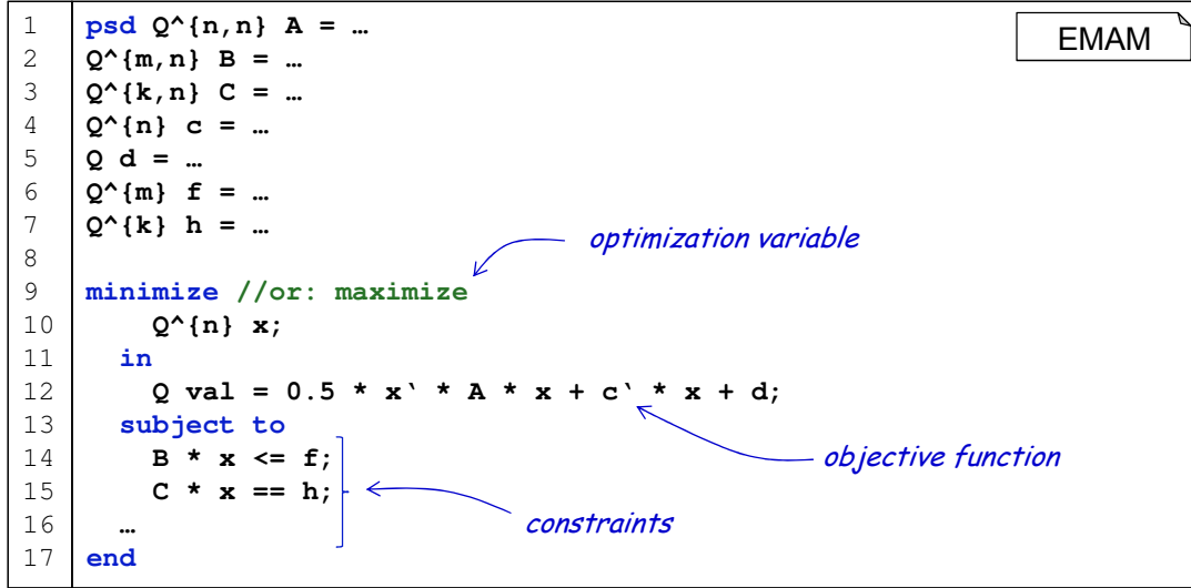
Figure 2.14: A MontiMath optimization statement representing a quadratic problem.
