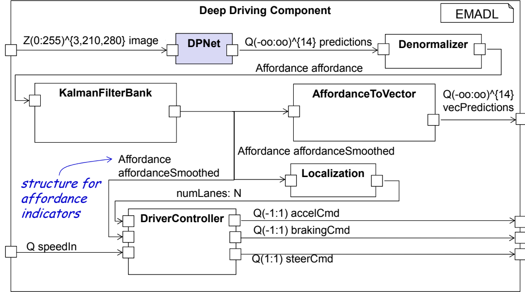
Figure 4.29: The deep direct perception-based architecture of a racing vehicle controller for TORCS [KPRS19].
