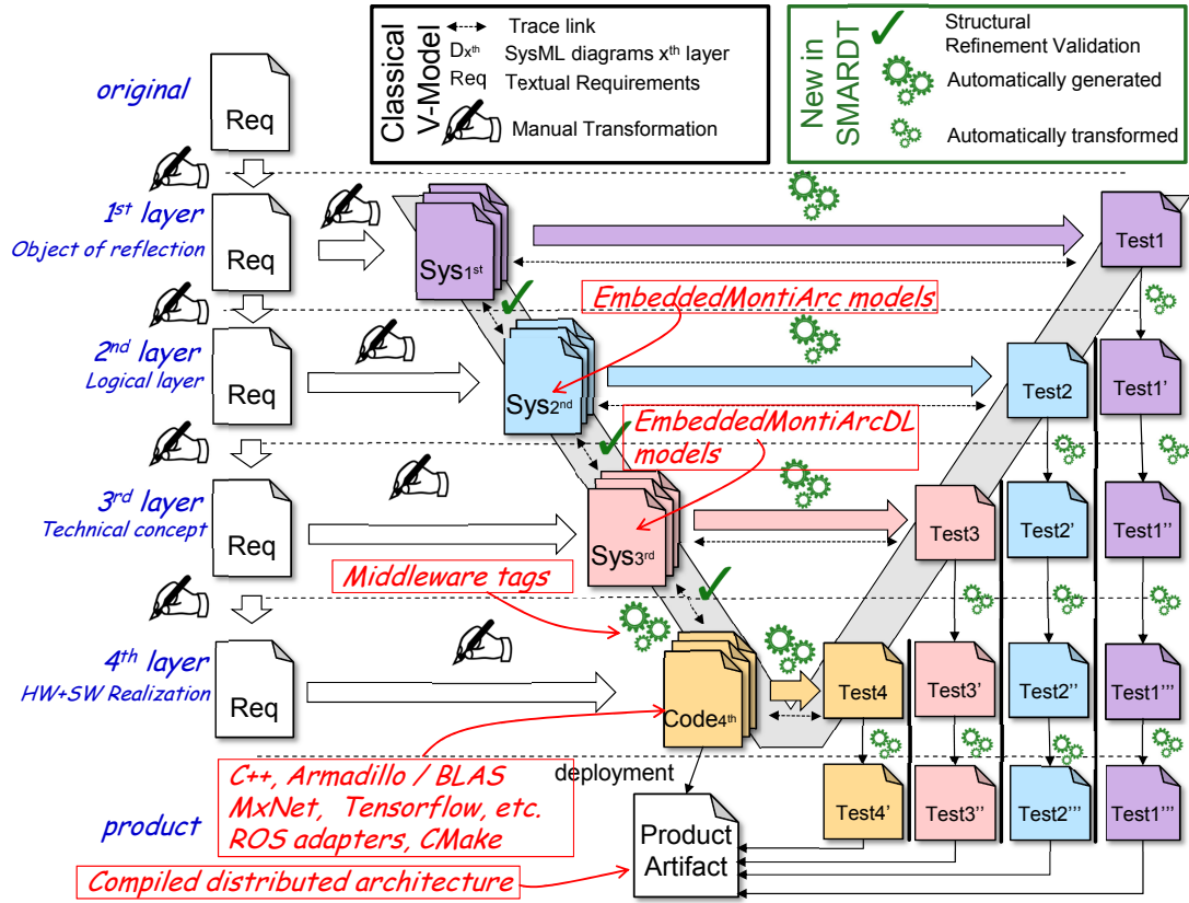
Figure 7.1: EMA in the SMaRDT process.
