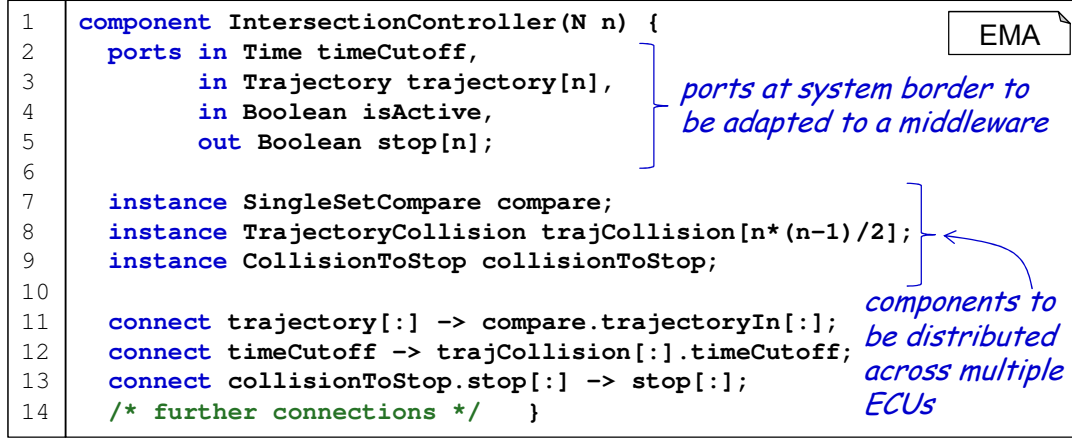
Figure 6.1: EMA definition of an intersection controller component receiving trajectories from nearby vehicles, checking for potential collisions and sending stop signals to endangered vehicles [HKKR19].
