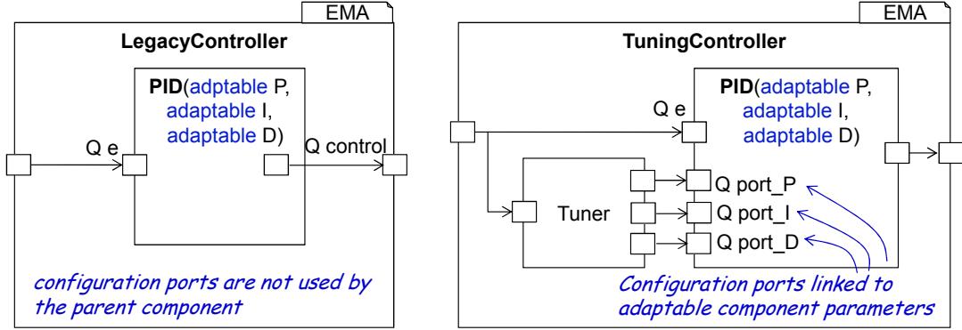
Figure 2.18: The components LegacyController and TunableController depict the static and the adaptable usage of the same PID component.
