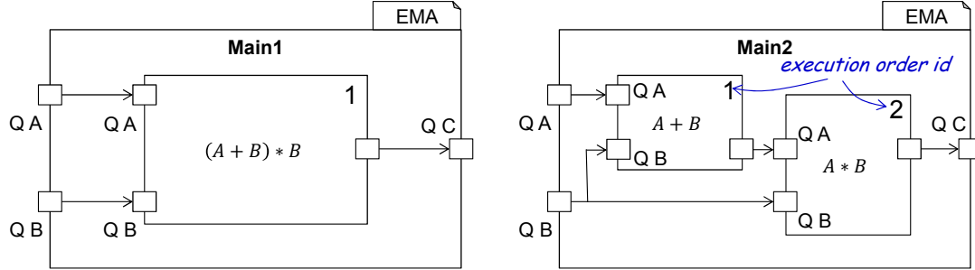
Figure 2.7: This example shows two C&C architectures Main1 and Main2, which are semantically equivalent in EMA due to its synchronized and weakly causal execution model, but which might have different interpretations in a language with strongly causal semantics.
