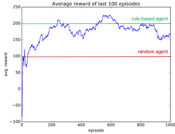
Figure B.2: Training results of the MontiAnna-based forestry 5.0 agent compared to a randomly acting and a rule-based agent. The experiments were conducted by Sascha Dewes in his bachelor's thesis.
