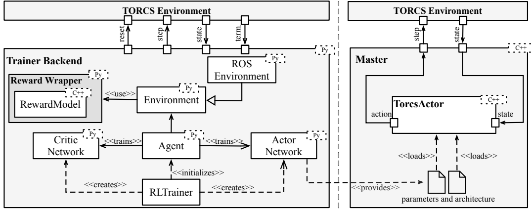
Figure 5.9: Generated artifacts: the left side shows the artifact architecture during the training. The right side is the artifact architecture at the execution time of the model [GKR19].
