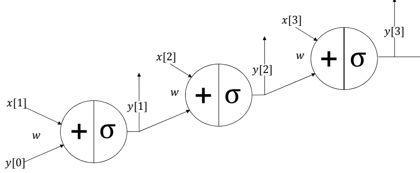
Figure 4.4: An RNN cell unfolded for three timesteps.
