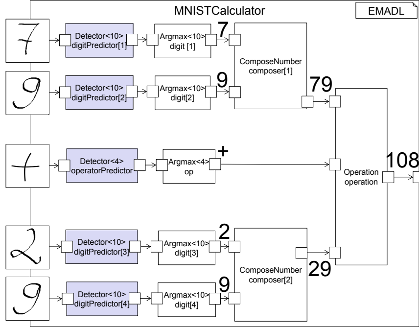
Figure 4.25: Component-and-connector architecture of an extended MNISTCalculator [KNP + 19].
