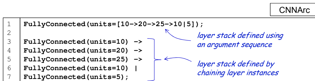
Figure 4.15: The definition of five fully connected layers with different numbers of units with and without an argument sequence.
