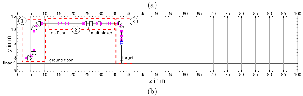
Figure 5.6.: Side view ( yz -plane, x into the image plane) of the top-level design of the HBS High-Energy Beam Transport (HEBT) beamline. A list with all elements and positions is given in appendix E. (a): Straight HEBT beamline. The drawing shows the three different sections and the respective quadrupole (pink), dipole (black), kicker (black) and beam scanner (blue) magnet positions. The multiplexer is located in the second section as indicated. The target is positioned 1.35 m above the ground floor. (b): Left HEBT beamline projected on the yz -plane. The first section and the first six quadrupoles of the second section are shared with the straight HEBT beamline and the third section is identical. In the second section, the beam passes the left arc of the multiplexer system (shown in detail in figure 5.1).
