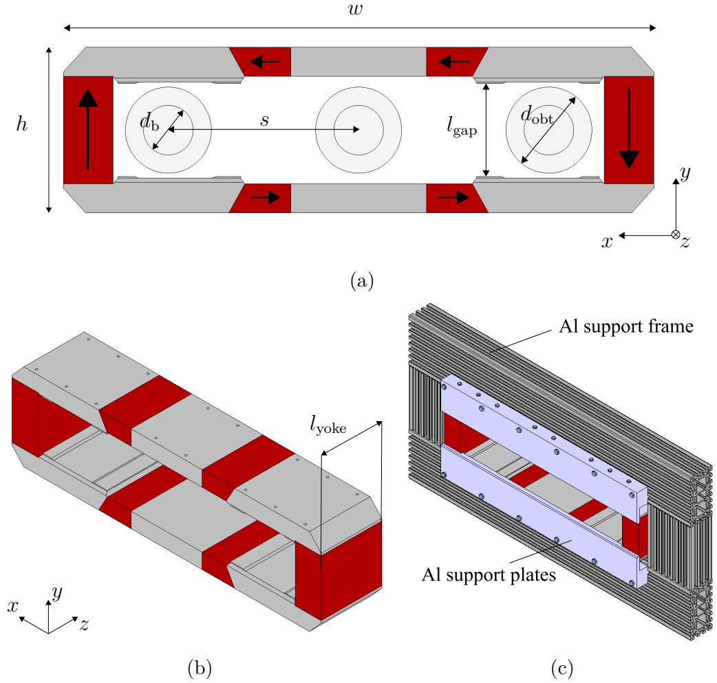
Figure 4.37.: (a): Technical layout of the TFM front face. The width of the front face is w = 714\text{ mm} and the height h amounts to 200\text{ mm} . The gap height l_{\text{gap}} = 112\text{ mm} allows to accommodate a beam tube with outer diameter d_{\text{obt}} = 104\text{ mm} . The expected beam diameter is d_b = 60\text{ mm} (6 rms beam widths according to figure 4.9). The separation of the beam spots is s = 230\text{ mm} . The red parts indicate SmCo magnets with B_r = 1.1\text{ T} , the gray parts show the magnet yoke. The magnetization directions of the permanent magnets are indicated with arrows. (b): Side view of the structure in (a) with a yoke length of l_{\text{yoke}} = 140\text{ mm} . (c): Full TFM setup with a customized Al support structure. Al support plates are mounted on the magnet yoke and connected to an Al support frame, which stabilizes the structure.
