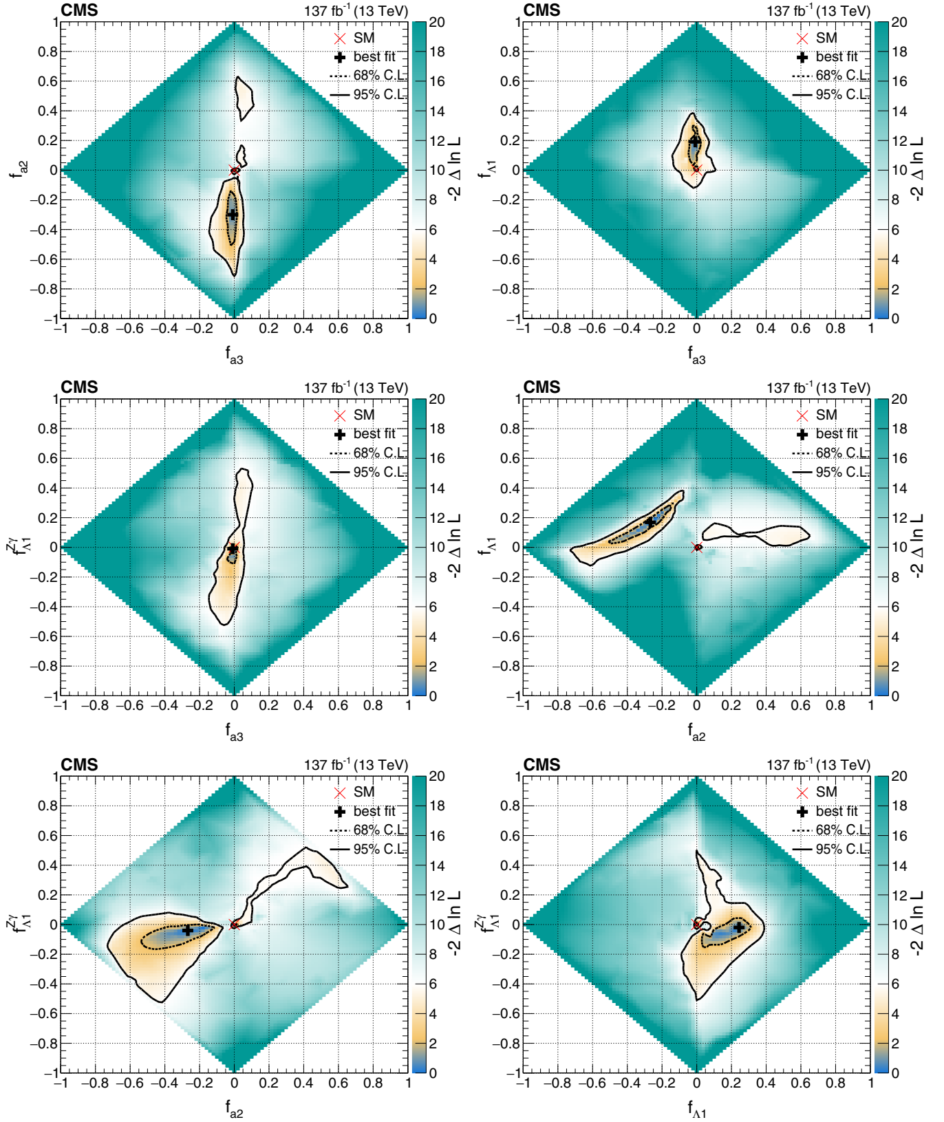
FIG. 19. Observed two-dimensional likelihood scans of the four coupling parameters f_{a3} , f_{a2} , f_{\Lambda 1} , and f_{\Lambda 1}^{Z\gamma} in approach 1 with the coupling relationship a_i^{WW} = a_i^{ZZ} . In each case, the other two anomalous couplings along with the signal strength parameters have been left unconstrained. The 68 and 95% CL regions are presented as contours with dashed and solid black lines, respectively. The best fit values and the SM expectations are indicated by markers.
