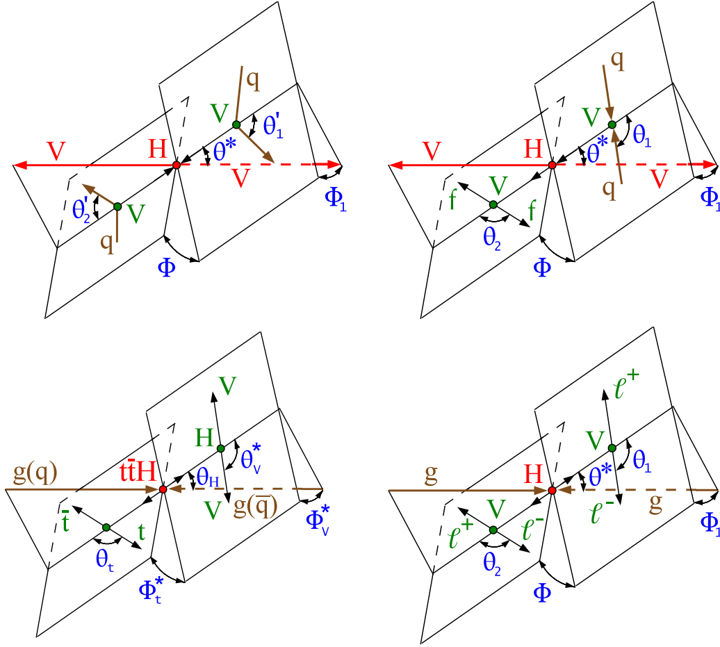
FIG. 8. Four topologies of the H boson production and decay: gluon or EW vector boson fusion qq \rightarrow V_1 V_2 (qq) \rightarrow H(qq) \rightarrow (VV)(qq) (upper left); associated production qq \rightarrow V \rightarrow VH \rightarrow (ff)(VV) (upper right); H boson production in association with the top quarks t\bar{t}H or tH (lower left); and four-lepton decay H \rightarrow VV \rightarrow 4\ell where the incoming gluons gg indicate the collision axis (lower right), and which proceeds either with or without associated particles. The incoming partons are shown in brown and the intermediate or final-state particles are shown in red and green. The angles characterizing kinematic distributions are shown in blue and are defined in the respective rest frames [29,31,32]. The subsequent top quark decay is not shown. See Ref. [32] for details.
