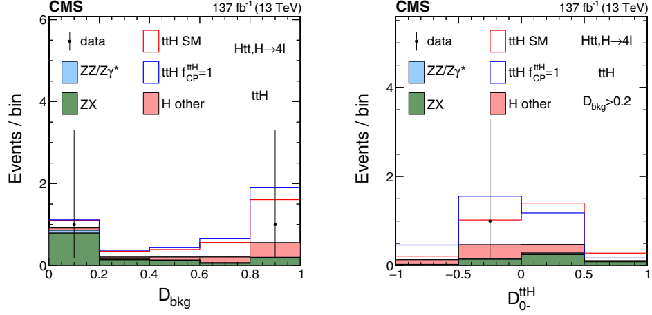
FIG. 9. Distribution of the \mathcal{D}_{\text{bkg}} (left) and \mathcal{D}_{0-}^{\text{ttH}} (right), discriminants in the sum of the \text{ttH} -leptonic and \text{ttH} -hadronic categories in scheme 1. The latter distribution is shown with the requirement \mathcal{D}_{\text{bkg}} > 0.2 in order to enhance the signal over the background contribution.
