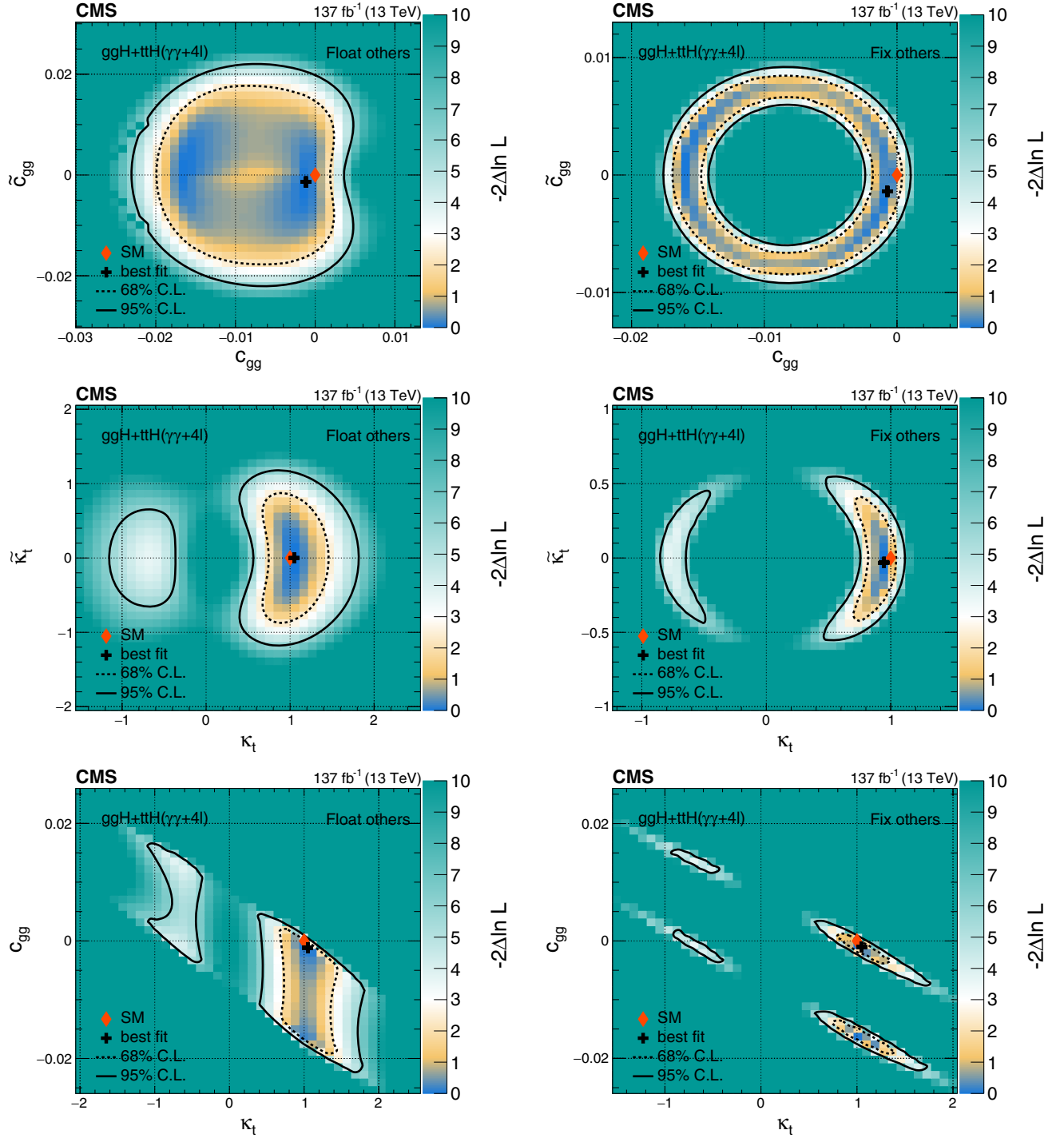
FIG. 17. Constraints on the anomalous H boson couplings c_{gg} , \tilde{c}_{gg} , \kappa_t , and \tilde{\kappa}_t in the t\bar{t}H , tH , and ggH processes combined, using the H \rightarrow 4\ell and \gamma\gamma decays. The constraints are shown for the pairs of parameters: c_{gg} and \tilde{c}_{gg} (upper), \kappa_t and \tilde{\kappa}_t (middle), \kappa_t and c_{gg} (lower), and with the other two parameters either profiled (left) or fixed to the SM expectation (right). The dashed and solid lines show the 68 and 95% CL exclusion regions in two dimensions, respectively.
