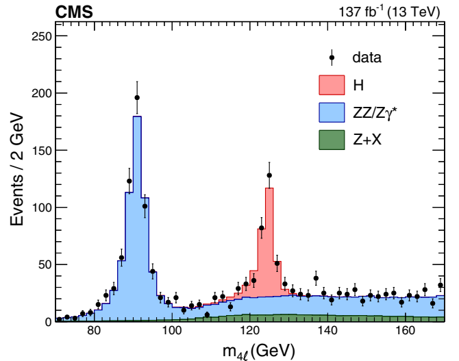
FIG. 6. Four-lepton invariant mass distribution of observed events (data points) and expectation from MC simulation or background estimates (histograms) in the region between 70 and 170 GeV [78]. The peaks from the Z and H \rightarrow 4\ell decays are visible near 91 and 125 GeV, respectively.
