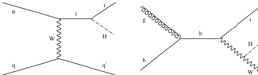
FIG. 4. Examples of leading-order Feynman diagrams for the tH production mode.
