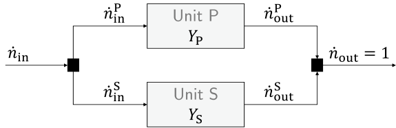
Fig. 1 Schematic of the simple example problem with the choice of producing a desired amount of a product, \dot{n}_{\text{out}} = 1 , either via Unit P ( Y_P = \text{True} , Y_S = \text{False} ) or Unit S ( Y_P = \text{False} , Y_S = \text{True} )
