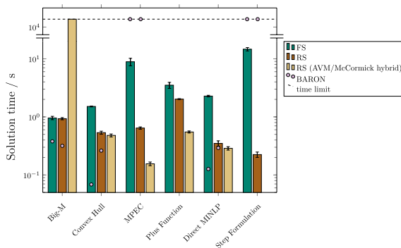
Fig. 7 Solution time for Problem (HEXGDP) using the problem formulations presented in Sect. 3 and the Step Formulation. As BARON can not handle max -functions, there are no results for the Plus Function. The solution times of the optimization with BARON and the MPEC and Step Formulation exceed the maximum solution time of 86400 s. No results are given for the RS (AVM/McCormick hybrid) Step Formulation, as it does not contain repeated nonlinear terms that could be replaced by AVs. The error bars represent the standard deviation from the arithmetic mean value of the solution time from 100 optimization runs using MAiNGO
