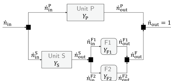
Fig. 2 Schematic of the flowsheet structure with two disjunctions and the choice of producing a desired amount of a product, \dot{n}_{\text{out}} = 1 , either via Unit P ( Y_{\text{P}} = 1, Y_{\text{S}} = 0 ) or Unit S ( Y_{\text{P}} = 0, Y_{\text{S}} = 1 ). If Unit S is chosen, the product needs to be further processed by either Unit F1 ( Y_{\text{F1}} = 1, Y_{\text{F2}} = 0 ) or F2 ( Y_{\text{F1}} = 0, Y_{\text{F2}} = 1 )
