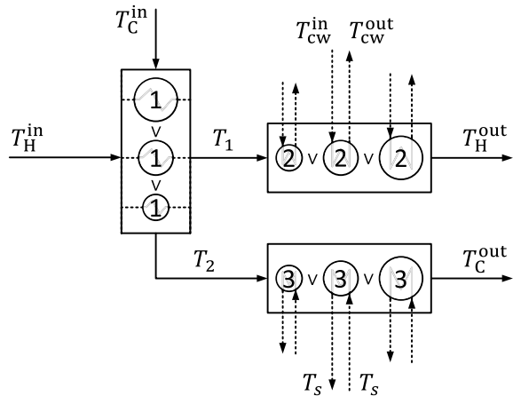
Fig. 6 Heat exchanger network based on the work of Türkay and Grossmann (1996a) with the choice between three different sizes for each heat exchanger 1–3
